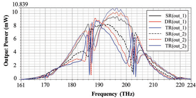
Fig. 4 Output results of ASK.
