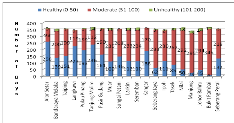
Figure 2: Air quality of west coast peninsular Malaysia, 2006 (DOE, 2007)
