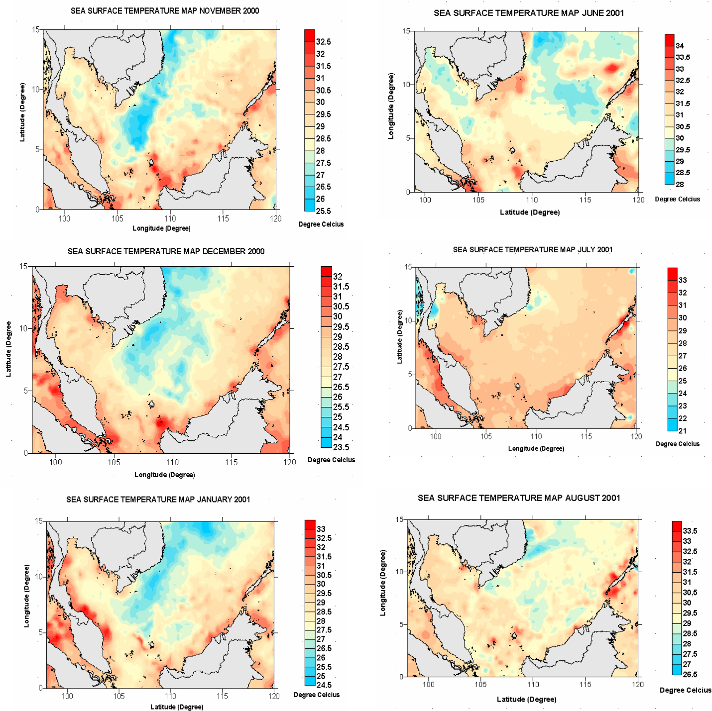
Figure 4(g). SST distribution during north east monsoon from Nov 2000 to Jan 2001.
