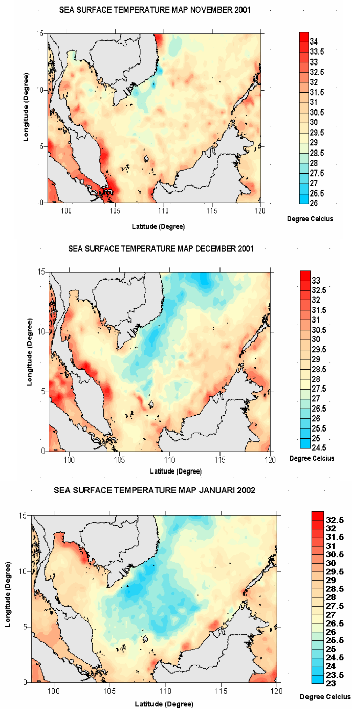
Figure 4(i). SST distribution during north east monsoon from Nov 2001 to Jan 2002.
