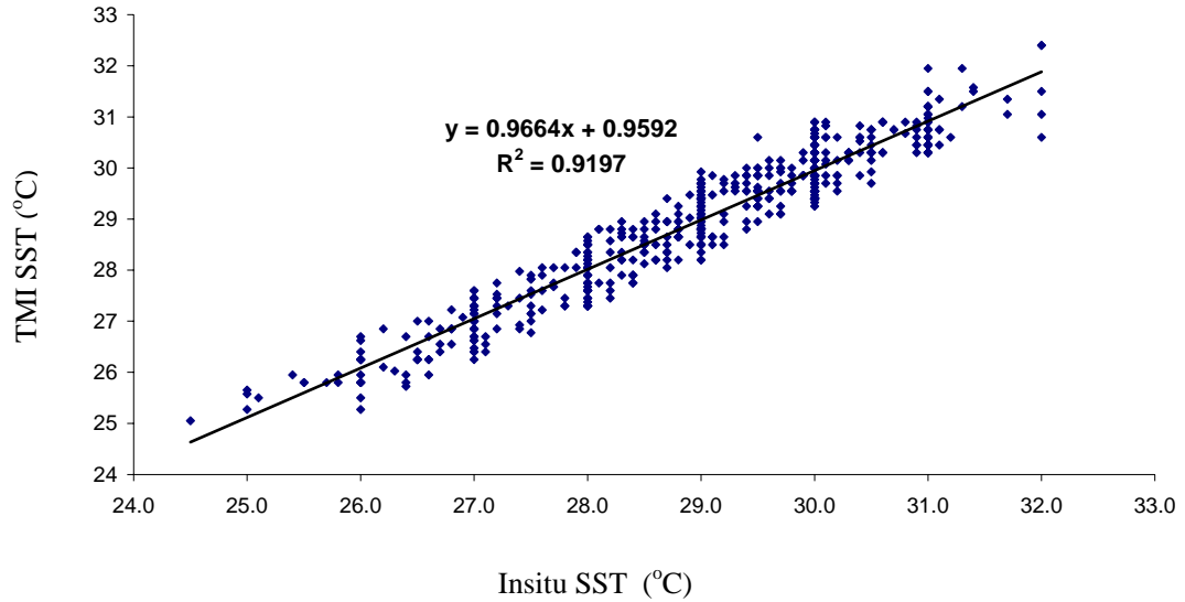
Figure 3. Regression of TMI SST versus in-situ SST from January 1998 to December 2002.
