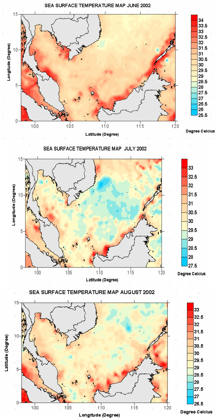
Figure 4(j). SST distribution during south west monsoon from June 2002 to Aug 2002.
