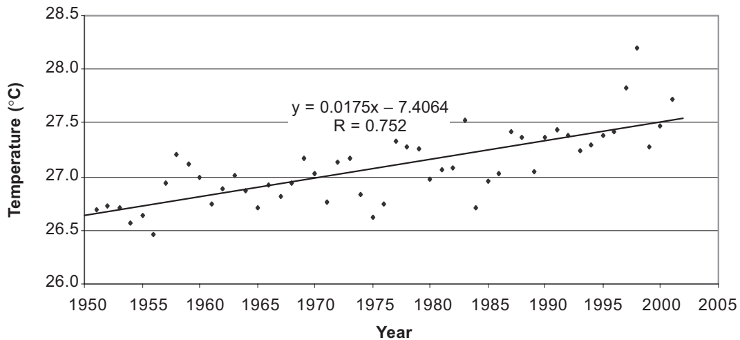
Figure 3 The regression line of the mean annual temperature of Penang from 1951-2001
