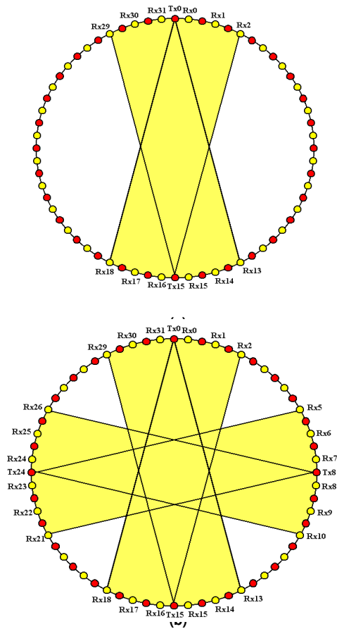
Figure 5: Multiple projection geometry a) 2-Projection b) 4-Projection
