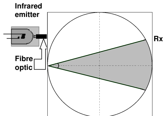
Figure 4: Determining emission angle.
