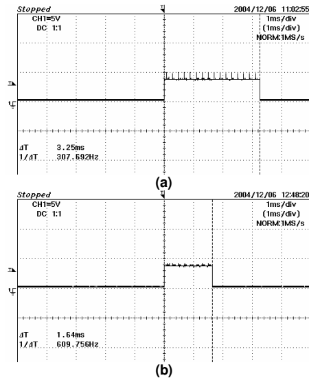
Figure 6: Total conversion time for one frame data a) 2-projection b) 4-projection
