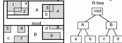
Fig. 6. R-Tree Indexing for 2 Dimension Bounding Box
