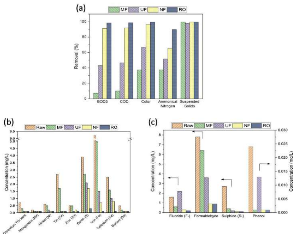
Fig. 5. In-depth analysis of the quality of leachate treated by different membranes, (a) general parameters, (b) metal-based parameters, and (c) other parameters (Note: pH of raw leachate: 8.4; pH of treated leachate: 8.6 (MF), 8.5 (UF), 8.6 (NF), and 9.1 (RO))
