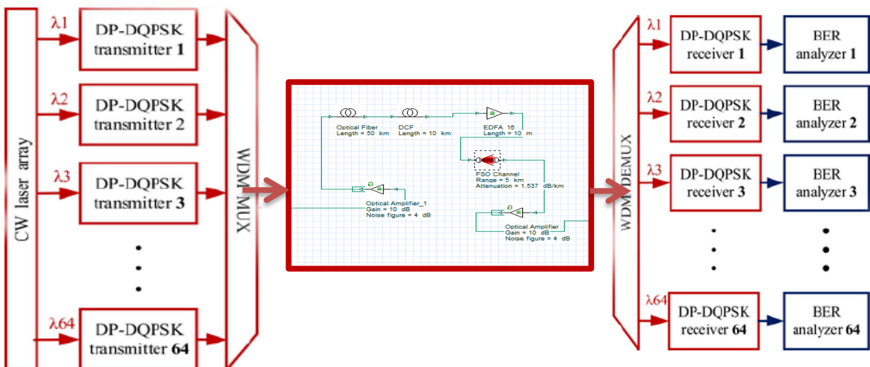
Figure 1. The schematic view of the proposed system design including the HOA and hybrid transmission medium
