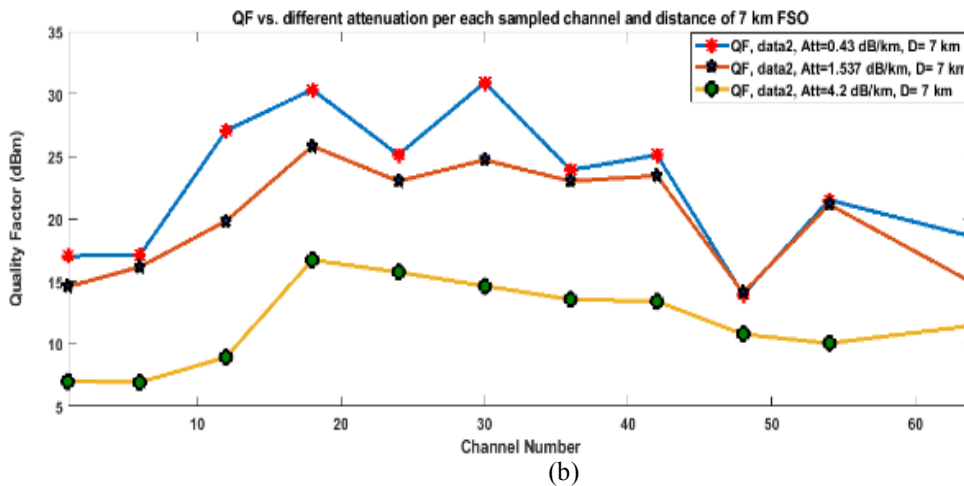
Figure 4. QF vs. different attenuation impacts for a distance of 7 km: (a) data 1, (b) data 2.
