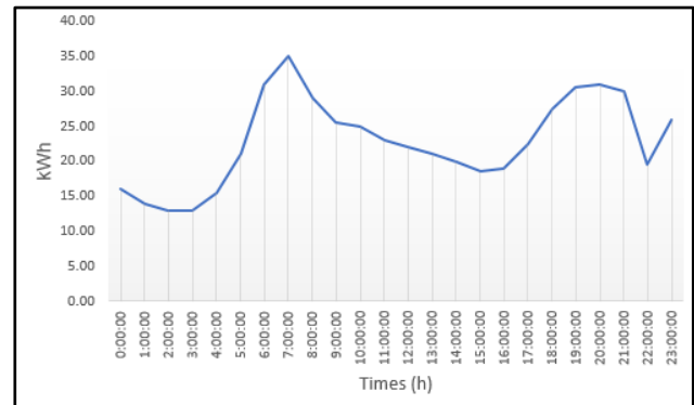
Figure 3 Hourly average load demand for simulation study
