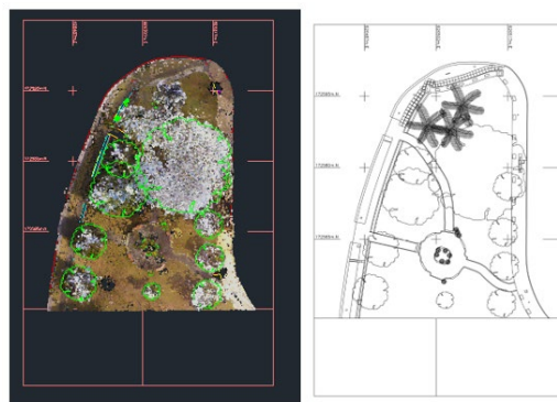
Figure 2.3 Side-by-side aerial view of 3D point cloud and digitized based map and been converted into a portable document format
