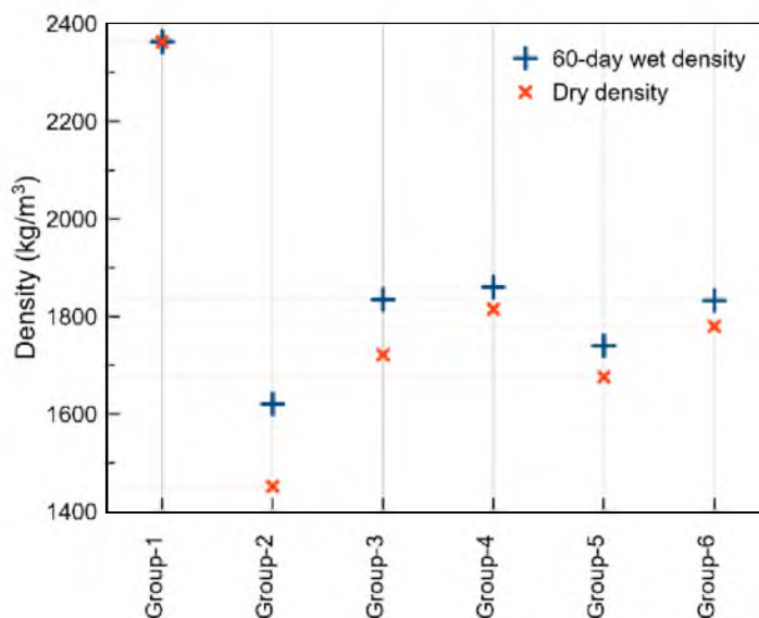
Fig. 6. Dry density versus wet density of concrete specimens
