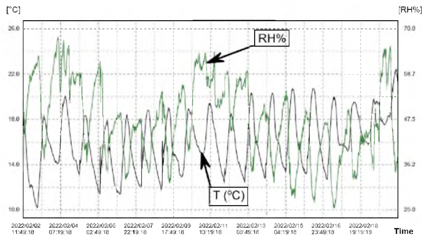
Fig. 4. Monitoring the temperature T (°C) and relative humidity RH (%) during the drying process of the coated (treated) wood shavings
