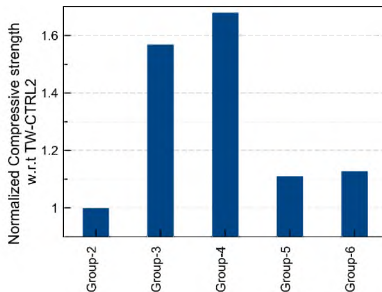
Fig. 9. Normalized compressive strength of the concrete made from wood shavings as coarse aggregate with respect to (w.r.t) Group-2 (TW-CTRL2)
