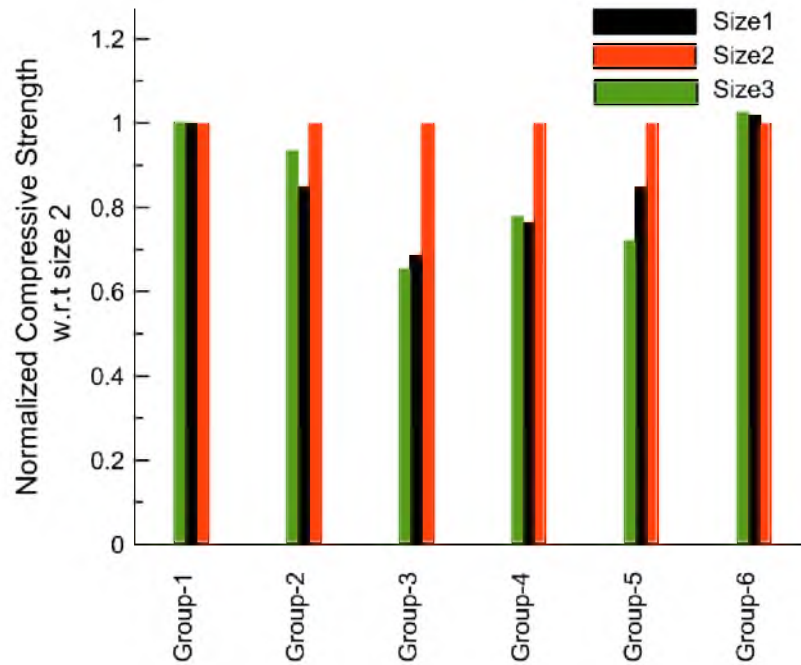
Fig. 10. Effect of the size of the specimen on the 28-day compressive strength of concrete
