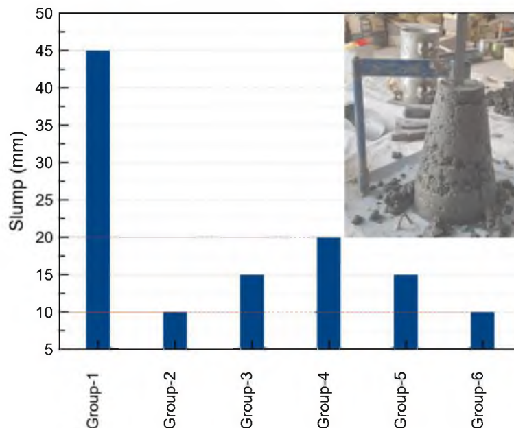
Fig. 5. Slump of fresh concrete of the six groups; Group-1 (NC-CTRL1), Group-2 (TW-CTRL2), Group-3 (CBTW-NE), Group-4 (CBTW-WE), Group-5 (ABTW-NE), and Group-6 (ABTW-WE)
