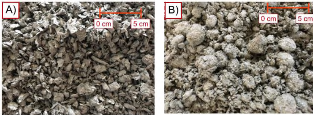
Fig. 2. Coating process of the wood shavings: A) cement paste coated wood shavings without emulsifier, B) Cement paste coated wood shavings with emulsifier
