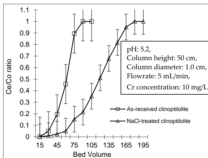
Figure 4. Breakthrough curve of as-received clinoptilolite and NaCl-treated clinoptilolite on Cr removal for the first run.
