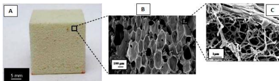
Fig. 3. A) Cubic specimen of RPU15 bio-foam, B) and C) FESEM images of the RPUF15 with different magnifications [31].
