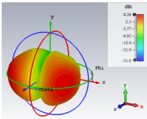
Figure 4. Simulated directivity frequency reconfigurable antenna OFF condition at 38 GHz
