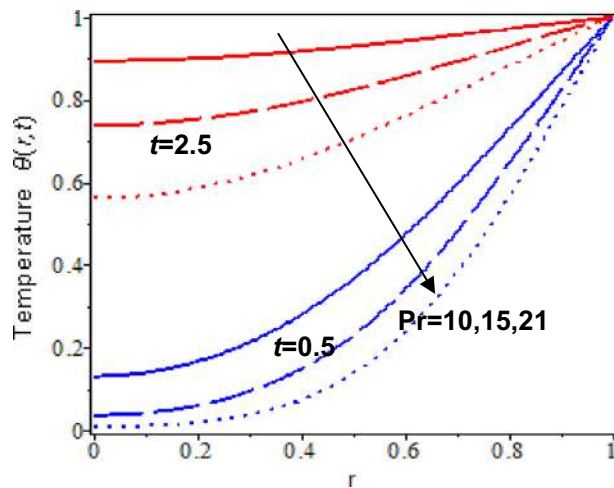
Figure 12. Nanofluid temperature with various Prandtl number and time parameter.
