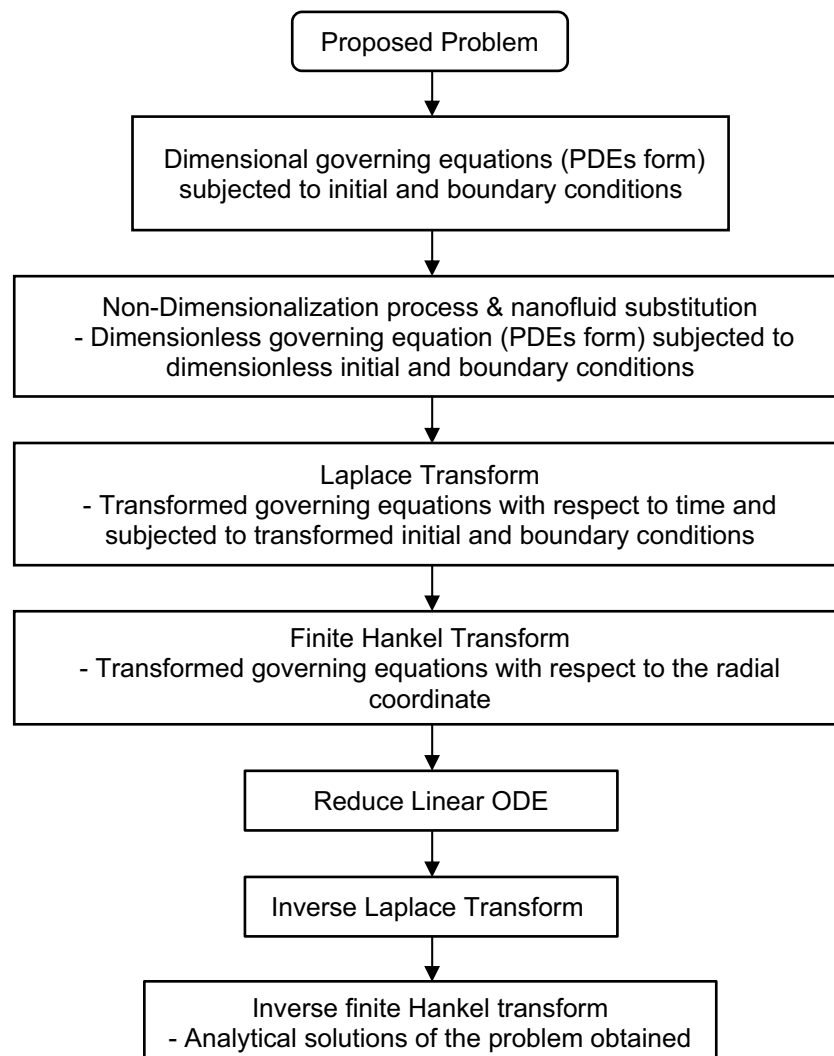
Figure 3. Methodology flowchart.
