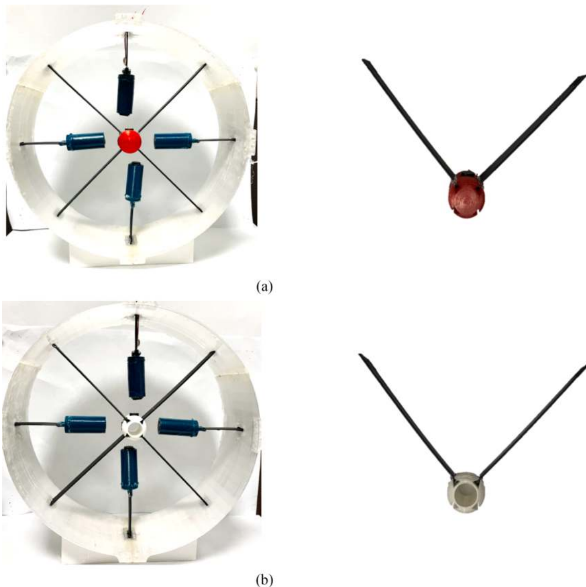
Fig. 7. Magnetically coupled energy harvester in top orientation: (a) Solid Coupler; (b) Hollow Coupler.
