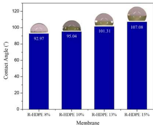
Fig. 5 Contact angles of the membranes.
