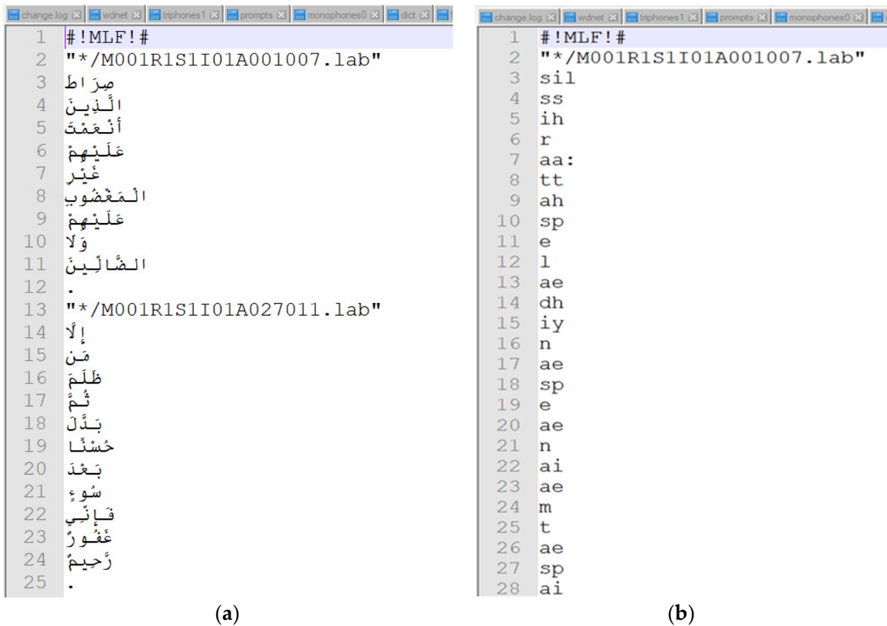
Figure 6. Sample of Level Transcriptions, (a) words Level Transcriptions, and (b) Phone Level Transcriptions.
