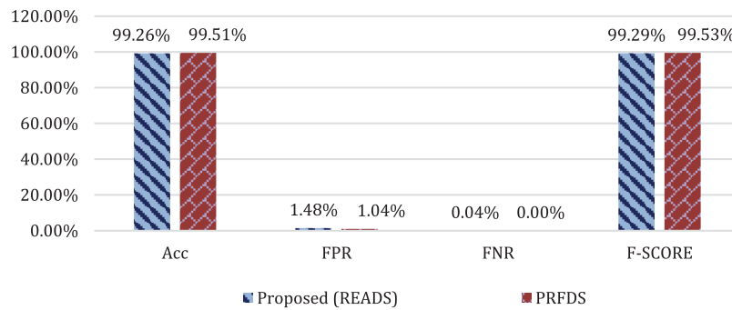
Figure 6: Results of proposed READS scheme (Attack scenario 1)
