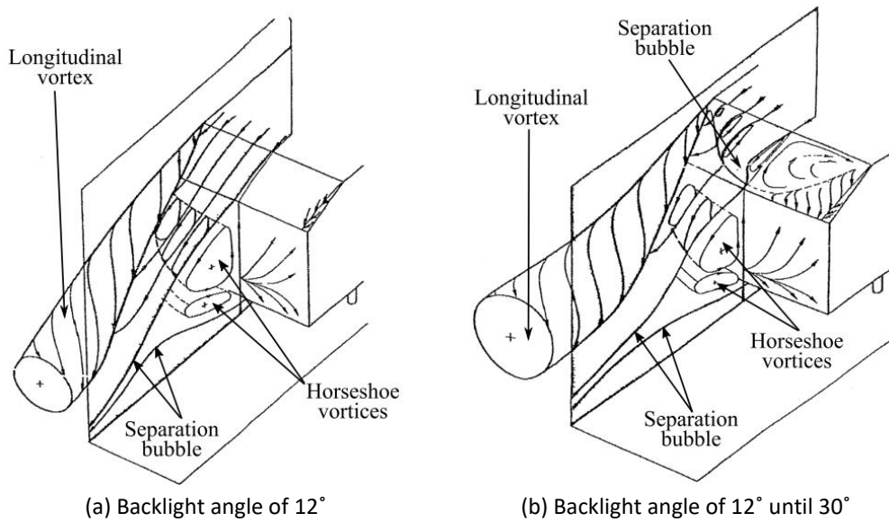
Fig. 2. The wake behind vehicle with backlight angle [8]
