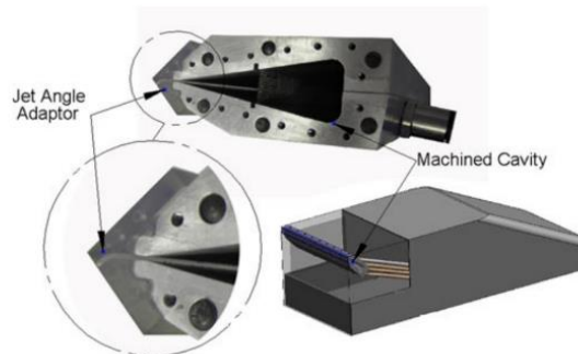
Fig. 6. Windsor model with blowing jet at the top of rear surface [16]
