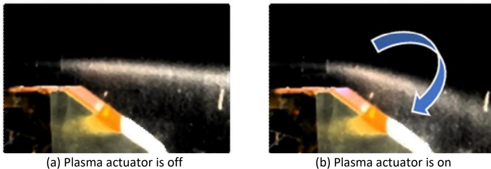
Fig. 5. Particle flow visualization at the back of Ahmed model installed with plasma actuator [10]
