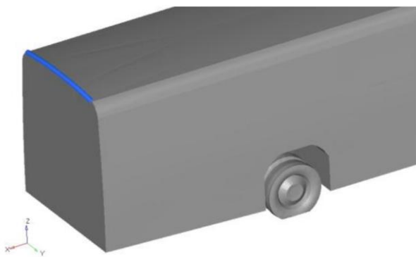
Fig. 20. Spoiler (blue) installed at roof end of bus mode [39]
