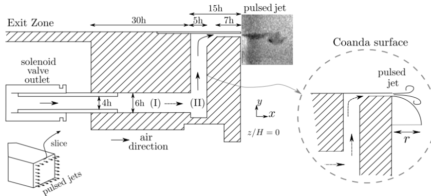
Fig. 12. Pulsed jet system attached at rear edges of vehicle [26]
