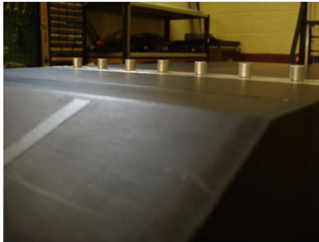
Fig. 30. Cylindrical VG used at rear roof of an Ahmed model with backlight angle [68]
