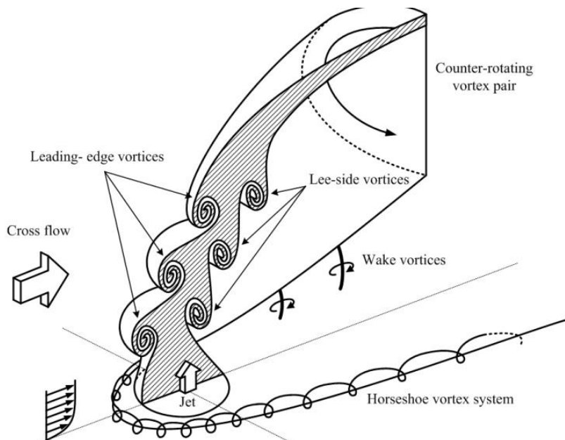
Fig. 11. Vortical structure produced by normal blowing jet [19]
