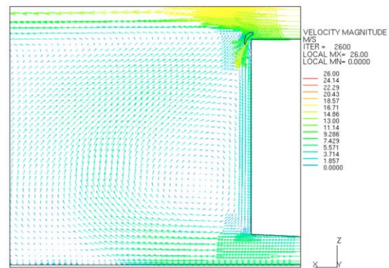
Fig. 21. Velocity plot at the back of bus with spoiler installed as viewed from side [39]
