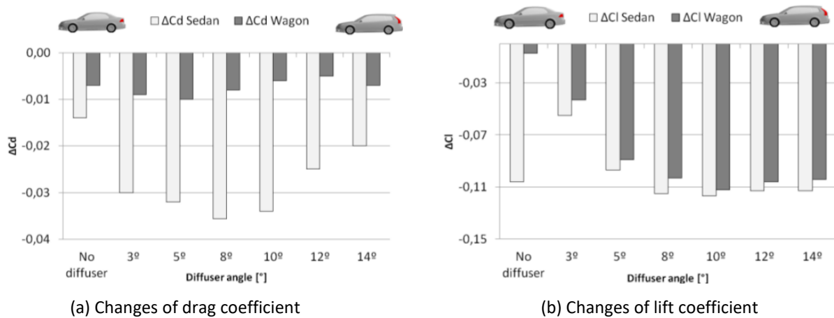
Fig. 22. Drag and lift coefficient changes due to diffuser angle [41]
