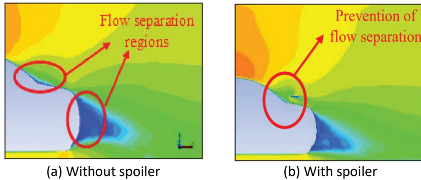
Fig. 15. Velocity contour at rear of Tata Manza model with and without spoiler [33]
