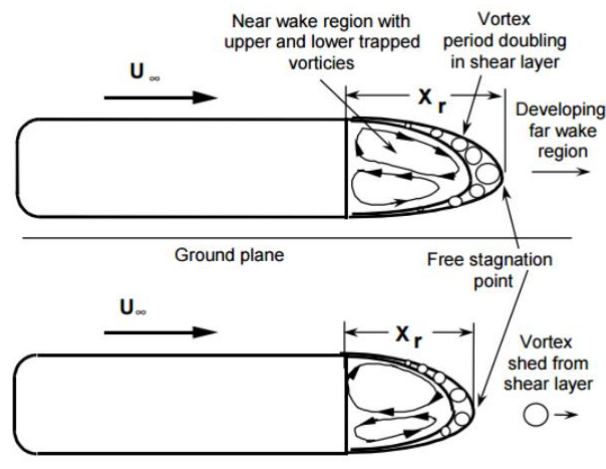
Fig. 3. The wake behind squareback vehicle along with its vortex shedding as viewed from side [9]
