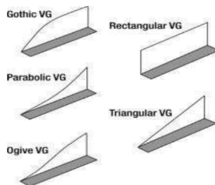
Fig. 31. Example of different profiles of VG used in research [70]
