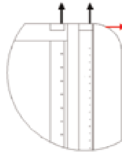
Fig. 8. Enlarged figure of orientation for actuator at rear edge of HSB where black and red arrows indicate normal and tangential blowing respectively [17]
