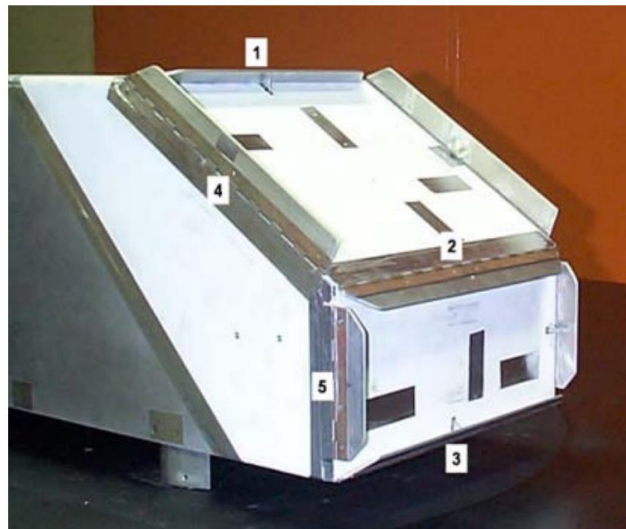
Fig. 27. Rear view of the Ahmed model installed with tail plates at edges [48]
