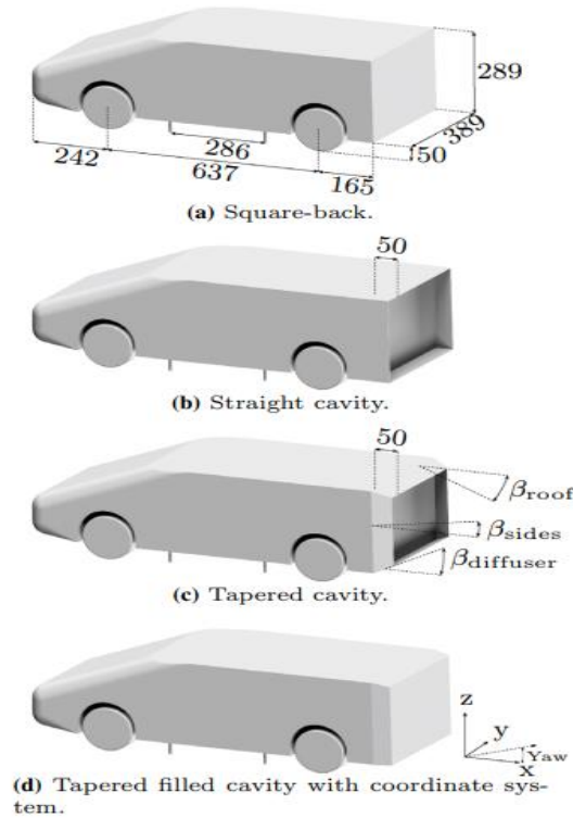
Fig. 26. Configuration of the Windsor model with rear extension used in the studies
