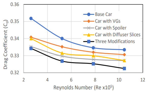
Fig. 33. Reduction of drag coefficient for different type of modifications of sedan car at different Re [34]
