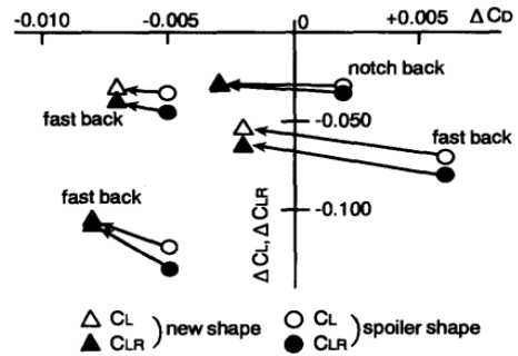
Fig. 19. Comparison of performance between new spoiler with conventional spoiler [38]
