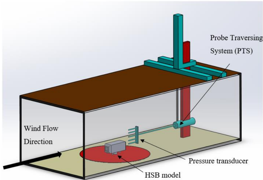
Fig. 37. Experiment setup in the Universiti Teknologi Malaysia-Low Speed Tunnel closed circuit
