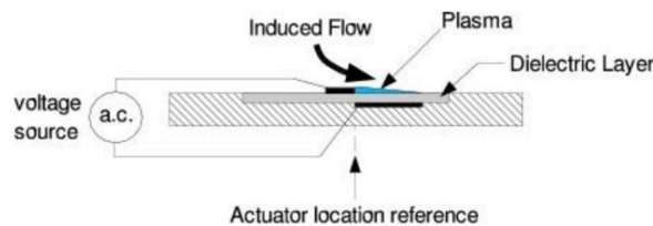
Fig. 4. Schematic drawing of SDBD plasma actuator [10]
