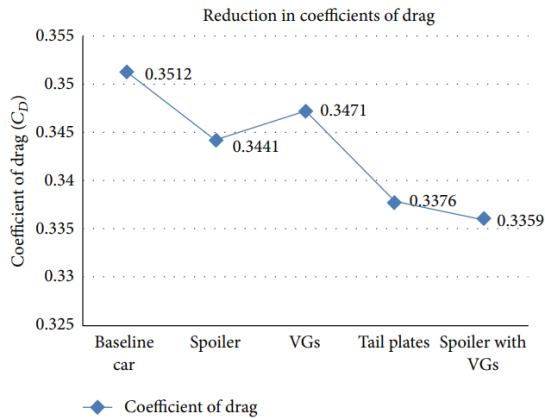
Fig. 32. Change of drag coefficient using different passive flow control [77]
