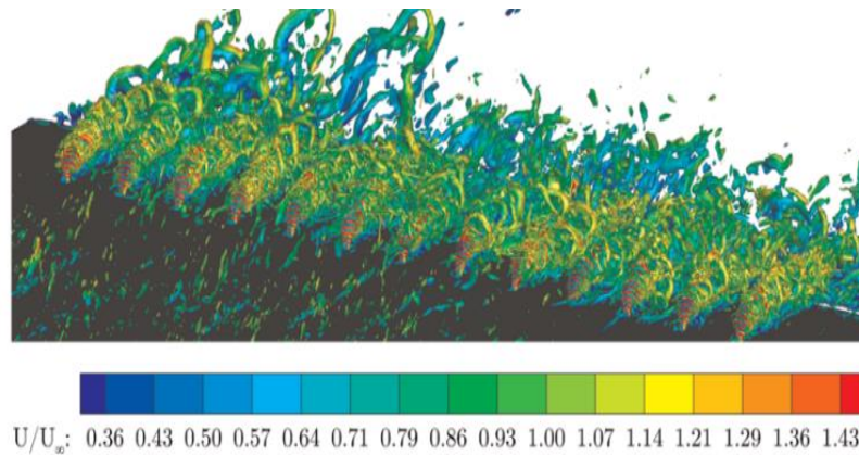
Fig. 10. Upstream view of microjets interacting with shear layer [17]
