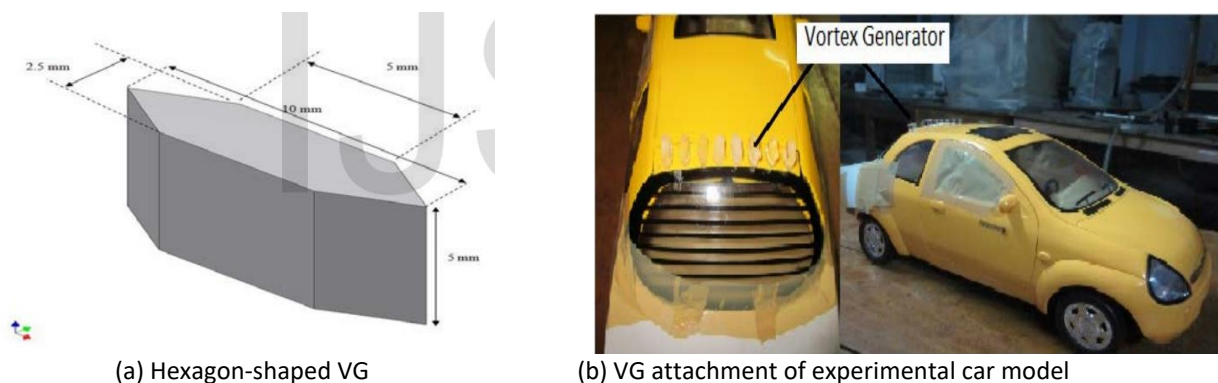
Fig. 29. Hexagon VG used in experimental study [67]
