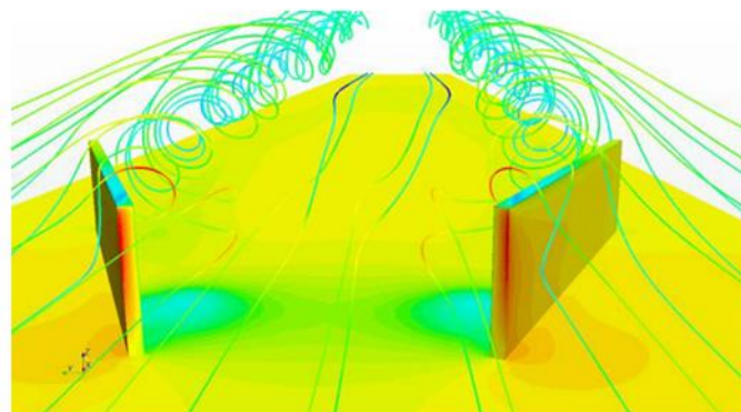
Fig. 28. Formation of vortices by rectangular plate VG [59]
