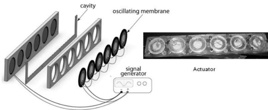
Fig. 13. Piezoelectric actuator used in experiment [30]
