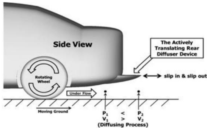
Fig. 25. Active diffuser installed under rear bumper of high-end car [45]
