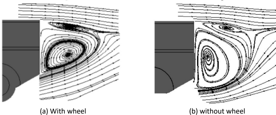
Fig. 24. PIV result at back of SUV model with wheel and without wheel [44]
