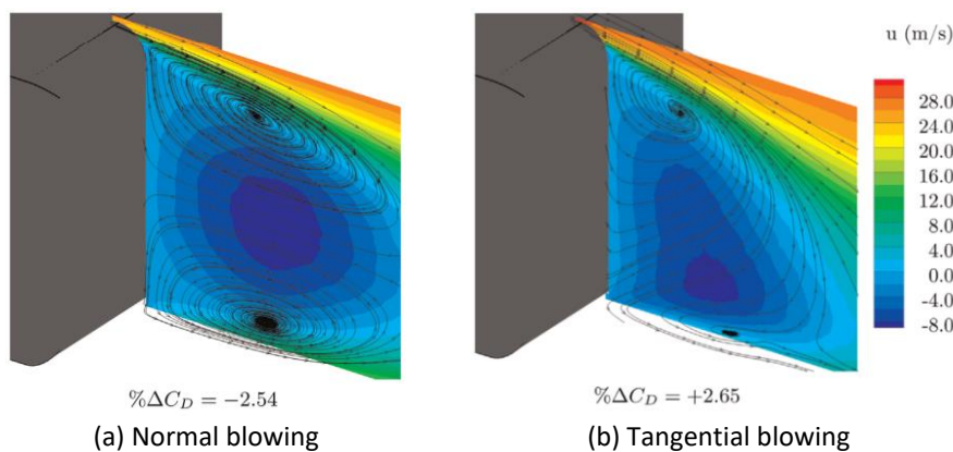
Fig. 9. The wake behind HSB with change of drag coefficient obtained using steady blowing [17]
