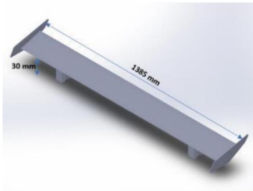
Fig. 16. The spoiler design used [34]
