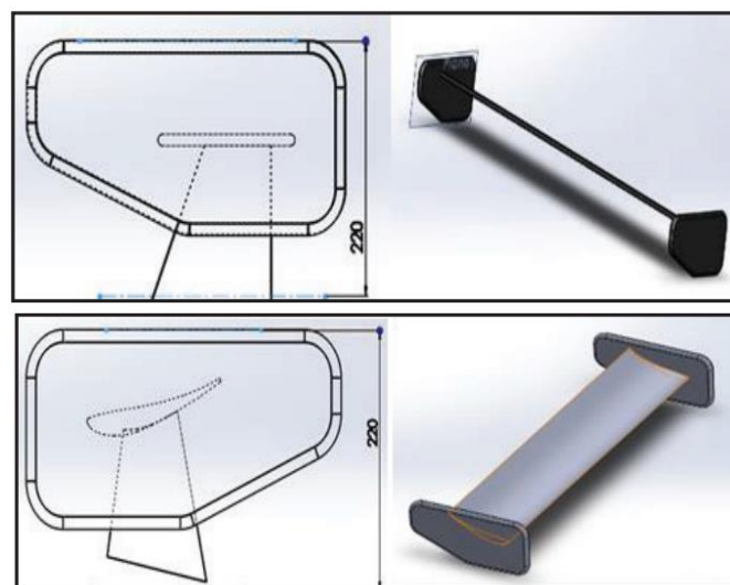
Fig. 14. Two design of spoilers that reduced drag on sedan vehicle [33]
