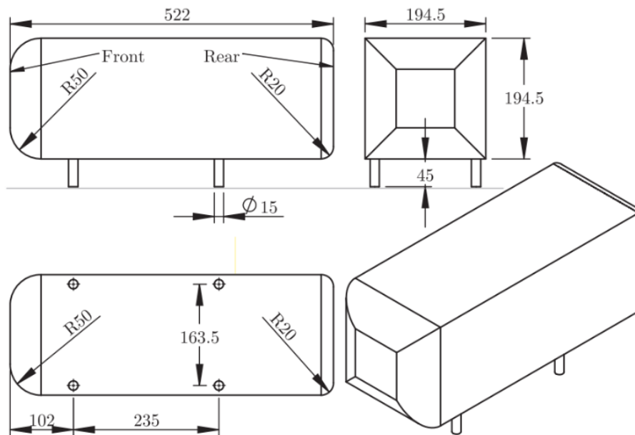
Fig. 35. Technical drawing of HSB with dimensions in mm
