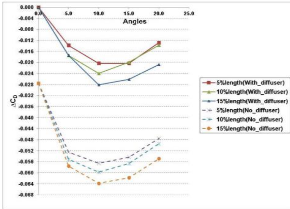
Fig. 23. Drag coefficient for squareback model with and without 10° diffuser along with tapering [42]
