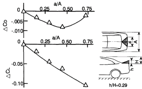
Fig. 18. Influence of spoiler dimension on aerodynamic coefficients of sedan car [38]
