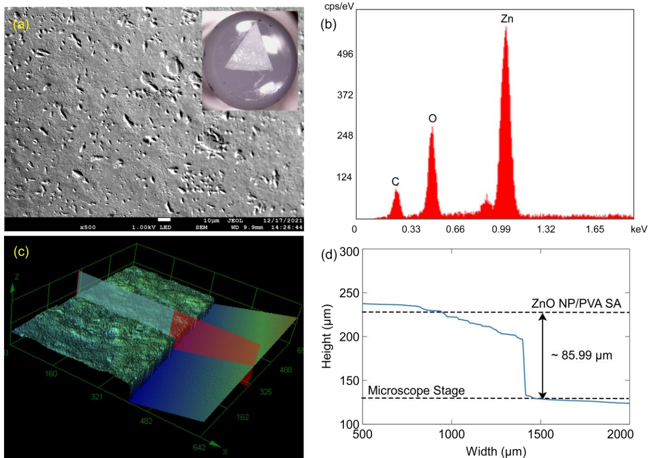
Fig. 2. ZnO NP/PVA film's (a) FESEM image (b) EDS spectrum (c) 3D thickness profile (d) Thickness measurement
