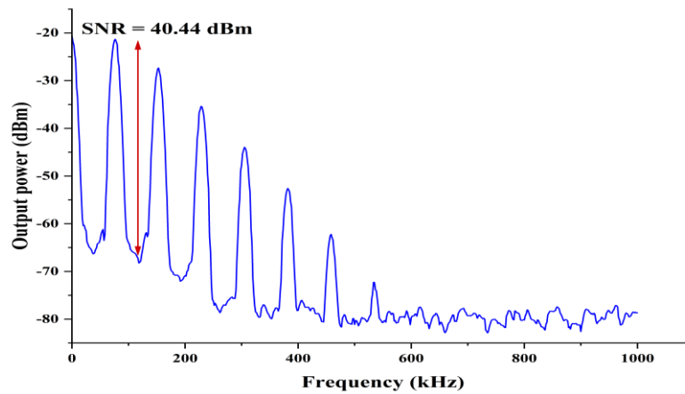
Fig. 8. RF spectrum of ZnO nanoparticles-PVA
