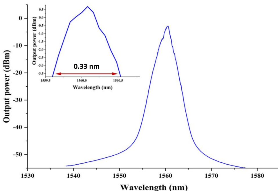
Fig. 4. Optical spectrum of the ZnO nanoparticles-PVA SA based Q-switched EDFL at 157.01 mW
