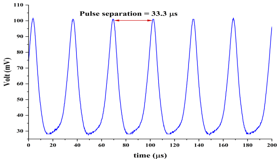
Fig. 5. Pulse train of ZnO nanoparticles-PVA SA based EDFL at 157.01 mW
