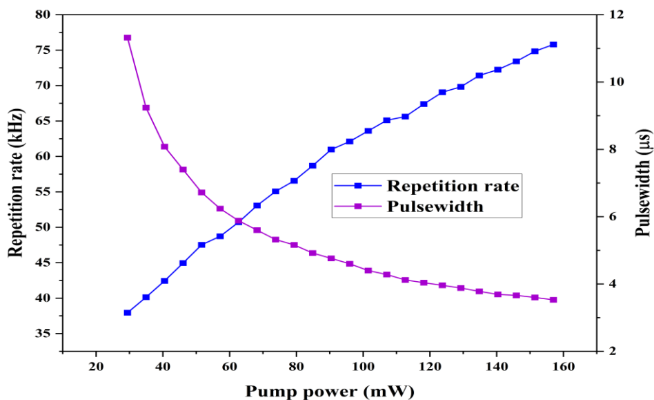
Fig. 6. Pulse width and repetition rate versus incident pump power
