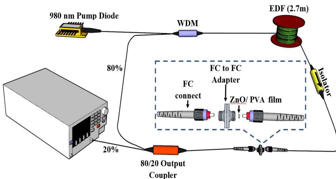
Fig. 3. Erbium-doped fiber laser set up the cavity
