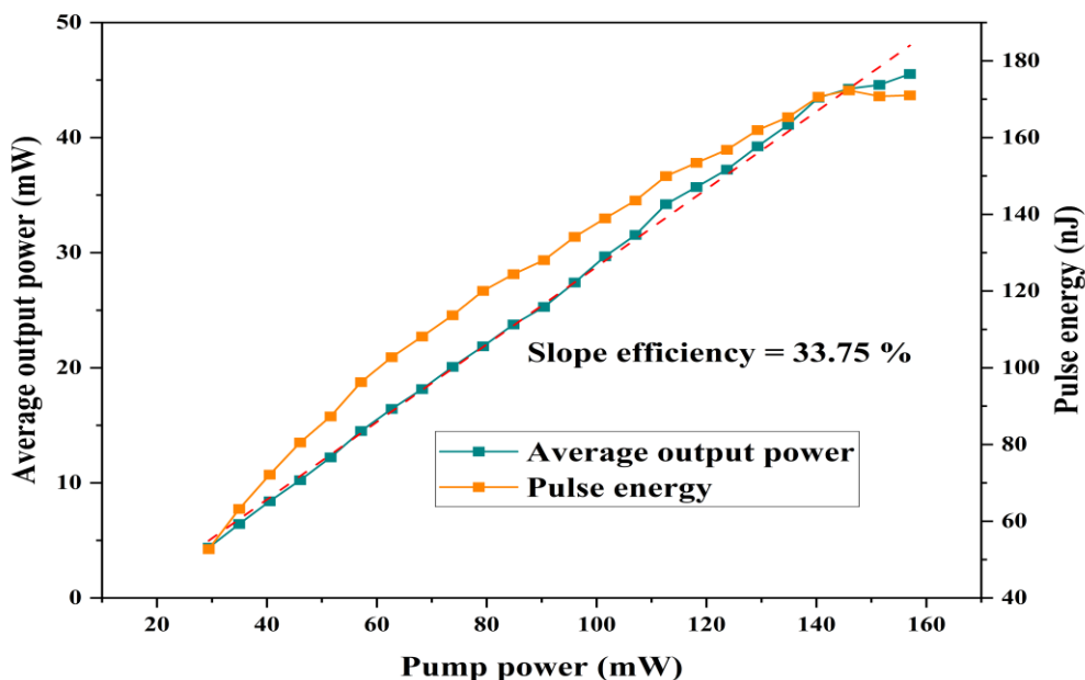
Fig. 7. Pulse energy and average output power versus incident pump power
