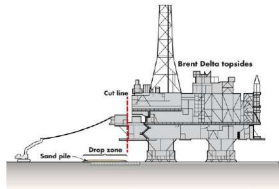
Fig. 4 Main structure dismantling process via cut and put method (Shell 2019)
