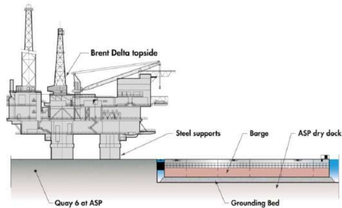
Fig. 3 Topside load-in operation (Shell 2019)
