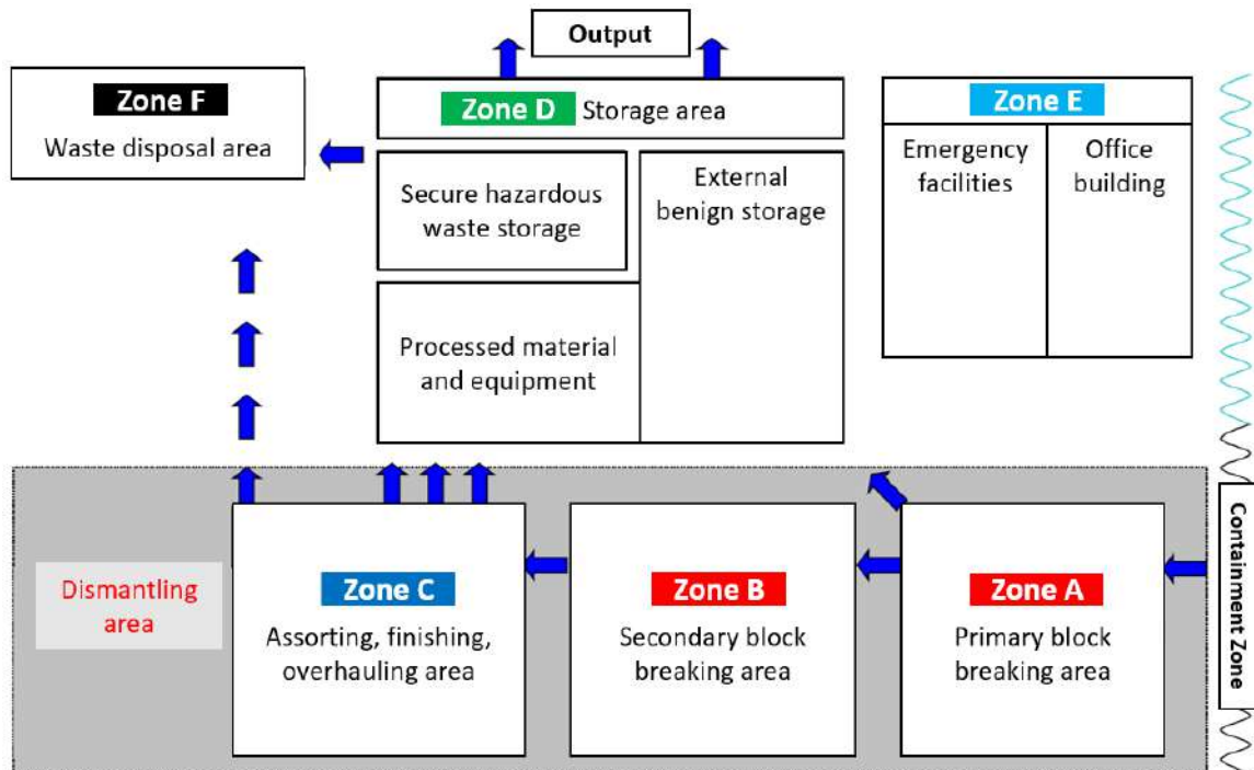
Fig. 5 Layout of ship recycling yard as suggested by UNEP (UNEP 2003)
