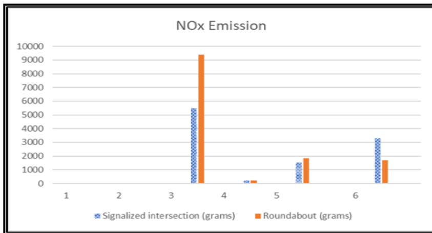
Fig. 14 - Vehicle emission results comparison (NOx)
