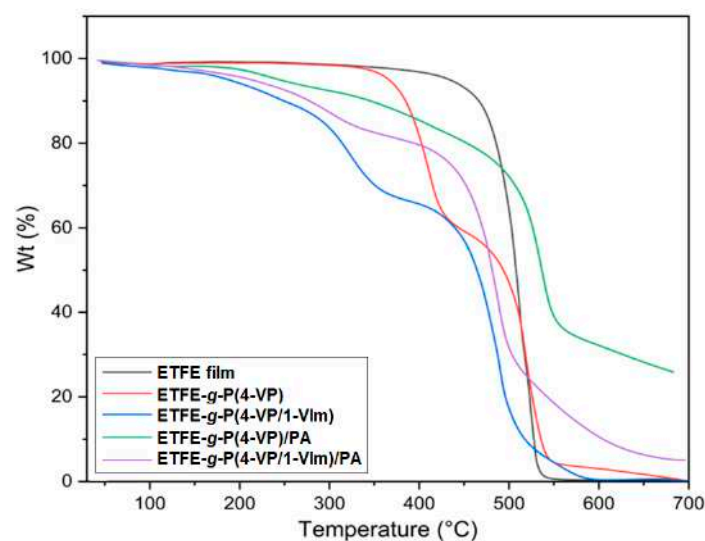
Figure 10. TGA thermograms of pristine ETFE film, ETFE-g-P(4-VP), and ETFE-g-P(4-VP/1-VIm) films compared to ETFE-g-P(4-VP)/PA and ETFE-g-P(4-VP/1-VIm)/PA membranes.
