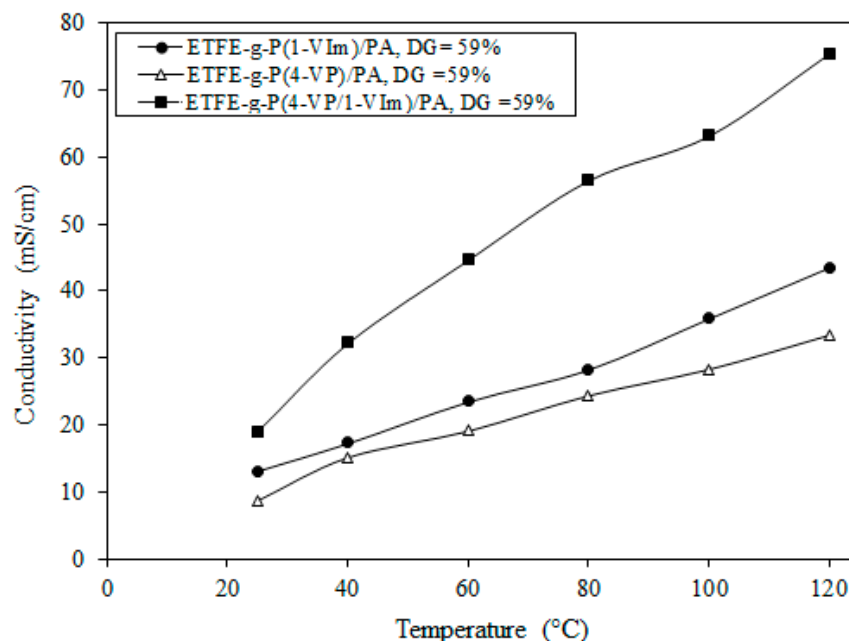
Figure 12. Variation of proton conductivity with temperature at anhydrous conditions for ETFE-g-P(4-VP/1-VIm)/PA compared to membranes obtained from the grafting of individual monomers.
