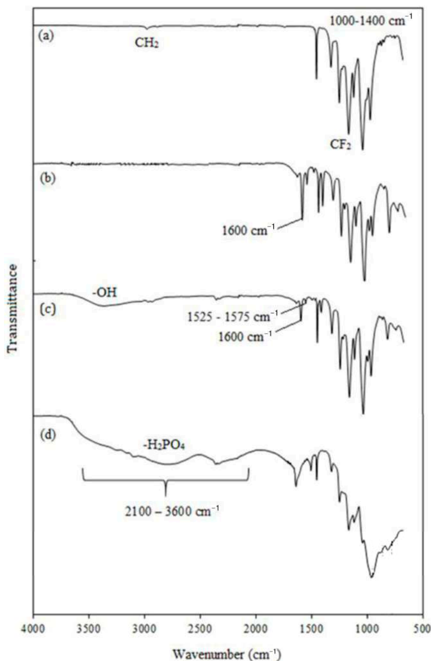
Figure 6. FTIR spectra of: (a) pristine ETFE film, (b) ETFE-g-P(4-VP) film, (c) ETFE-g-P(4-VP/1-VIm) film, and (d) ETFE-g-P(4-VP/1-VIm)/PA membrane with 59% DG.
