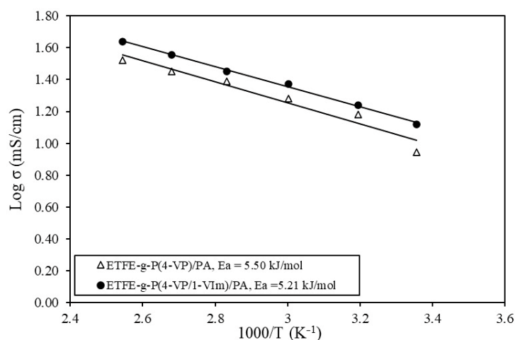
Figure 13. Arrhenius plots for proton conductivity vs. reciprocal of temperature for PA doped membranes.
