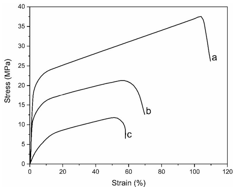
Figure 11. Stress-strain curves of: (a) pristine ETFE, (b) ETFE-g-P(4-VP/1-VIm)-grafted film, and (c) PA doped-membrane.
