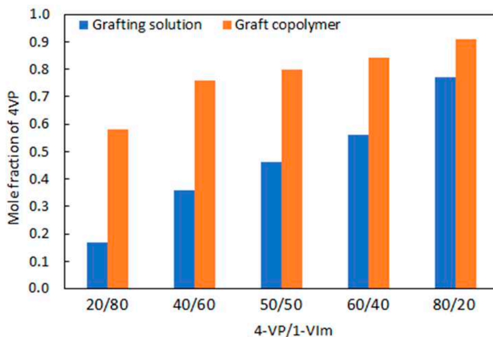
Figure 3. Variation of mole fraction of 4-VP in grafting mixture (blue) and in graft copolymer (orange). Grafting parameters: monomer conc. of 60 vol%, absorbed dose of 100 kGy, reaction time of 18 h, and temperature of 60 °C.
