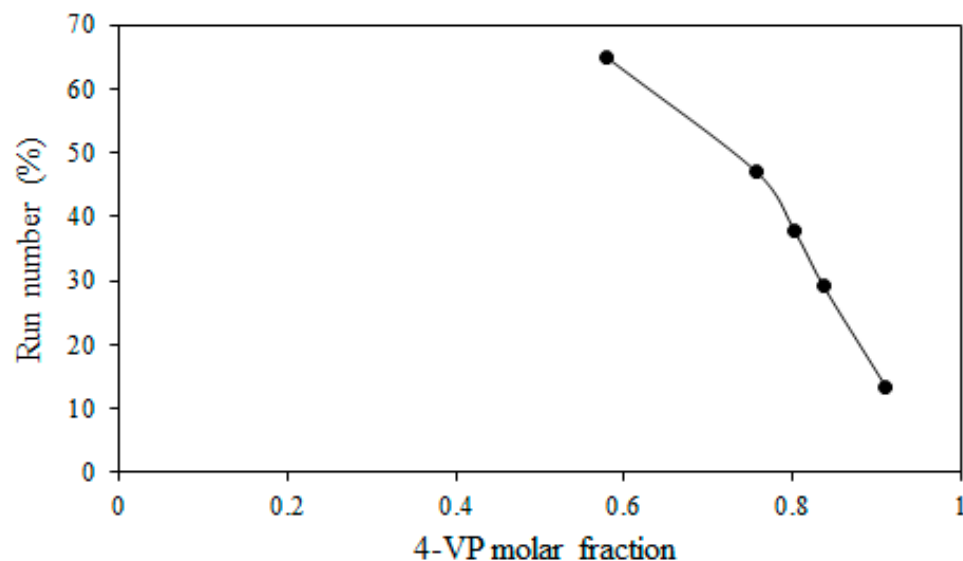
Figure 4. Variation of run number with 4-VP mole fraction in grafting of 4-VP/1-VIm mixtures onto ETFE film.
