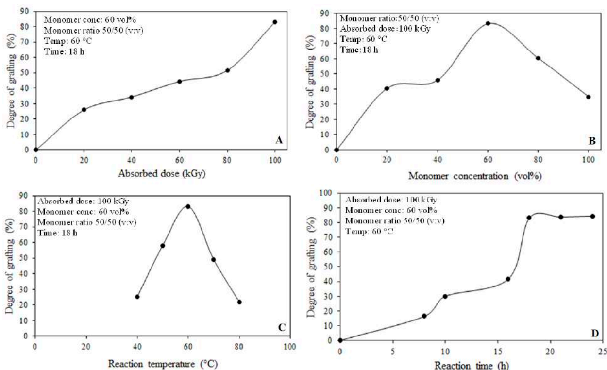
Figure 1. Variation of degree of grafting with reaction parameters: (A) absorbed dose, (B) monomer concentration, (C) reaction temperature, and (D) reaction time.
