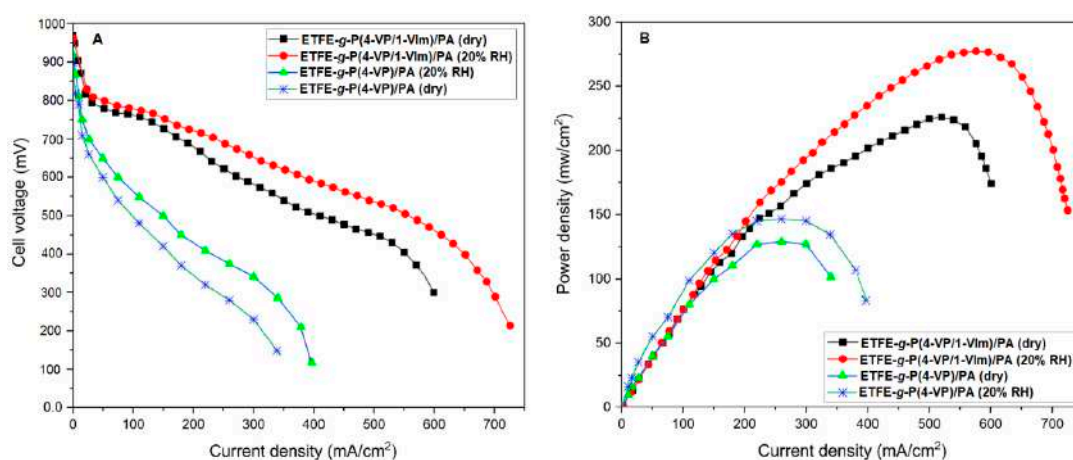
Figure 15. Performance of HT-PEMFC single cell with PA doped membranes (DG = 59% with a doping level of 119%): (A) polarization curves and (B) power density curves, tested under an anhydrous condition and 20% RH. \text{H}_2 flow rate is 450 mL/min and that of \text{O}_2 is 300 mL/min at temp. of 120 ^{\circ}\text{C} .
