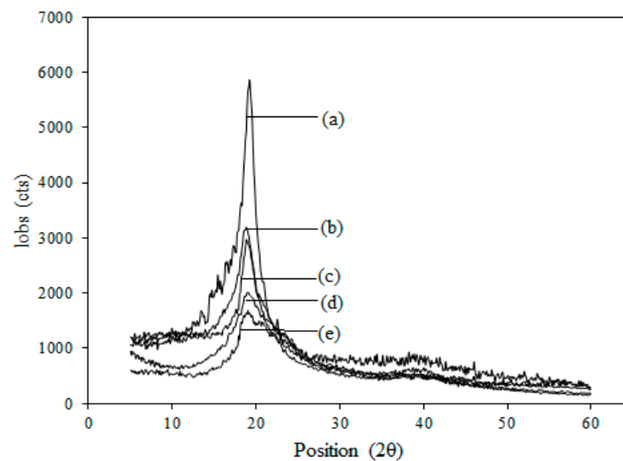
Figure 9. XRD diffractograms of: (a) pristine ETFE film, (b) ETFE-g-P(4-VP)-grafted film, (c) ETFE-g-P(4-VP/1-VIm)-grafted film, (d) acid-doped P(4-VP) membrane and (e) acid-doped P(4-VP/1-VIm) membrane.
