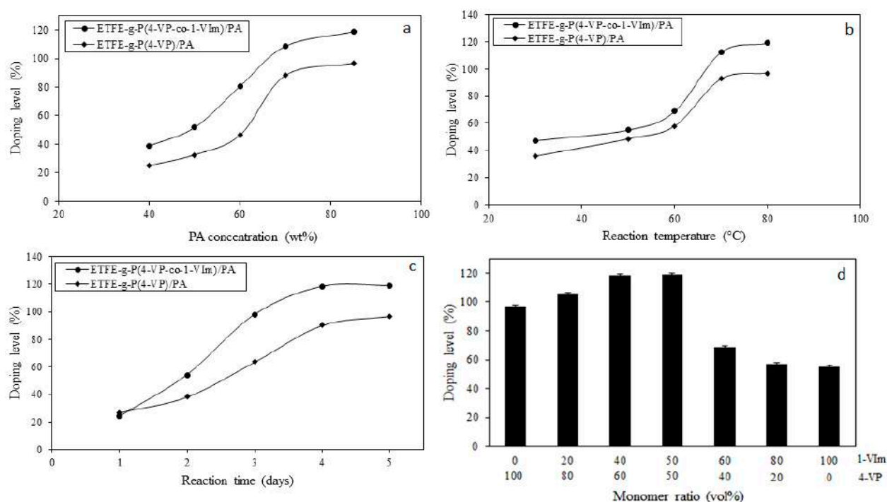
Figure 5. Variation of PA doping level of P(4-VP/1-VIm) grafted films with reaction parameters: (a) PA concentration, (b) reaction temperature, (c) reaction time, and (d) monomer ratio in grafting solution.
