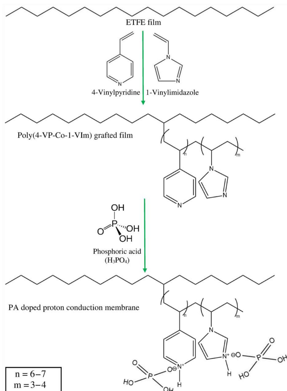
Figure 7. Schematic representation of preparation of PA-doped membrane obtained by RIGC of 4-VP/1-VIm mixture onto ETFE film.
