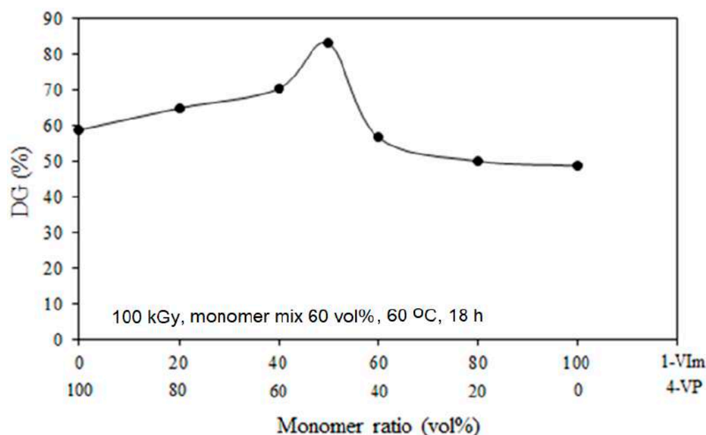
Figure 2. Variation of the degree of grafting with monomer ratio for grafting mixtures of 4-VP/1-VIm onto ETFE films.
