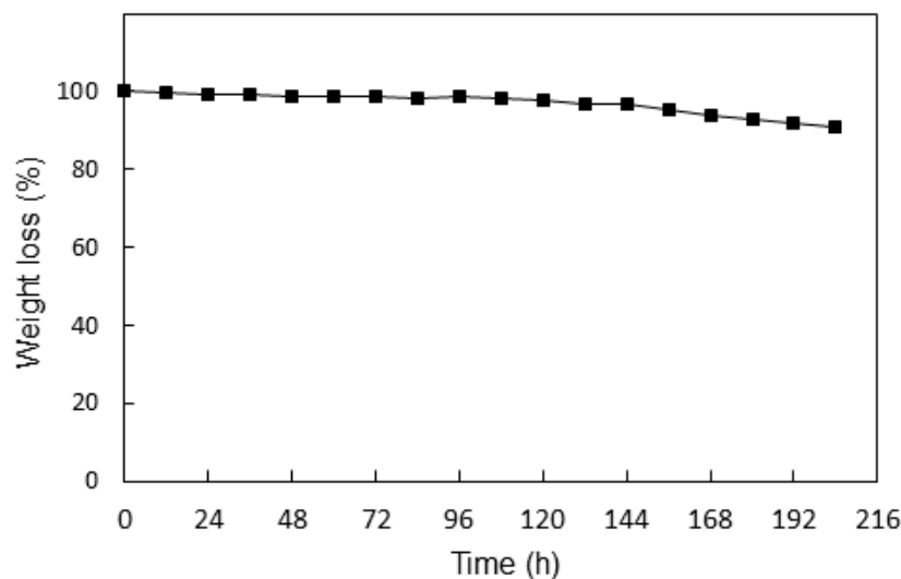
Figure 14. Variation of weight loss (%) with time during treatment of ETFE-g-P(4-VP/1-VIm)/PA membrane in Fenton reagent.
