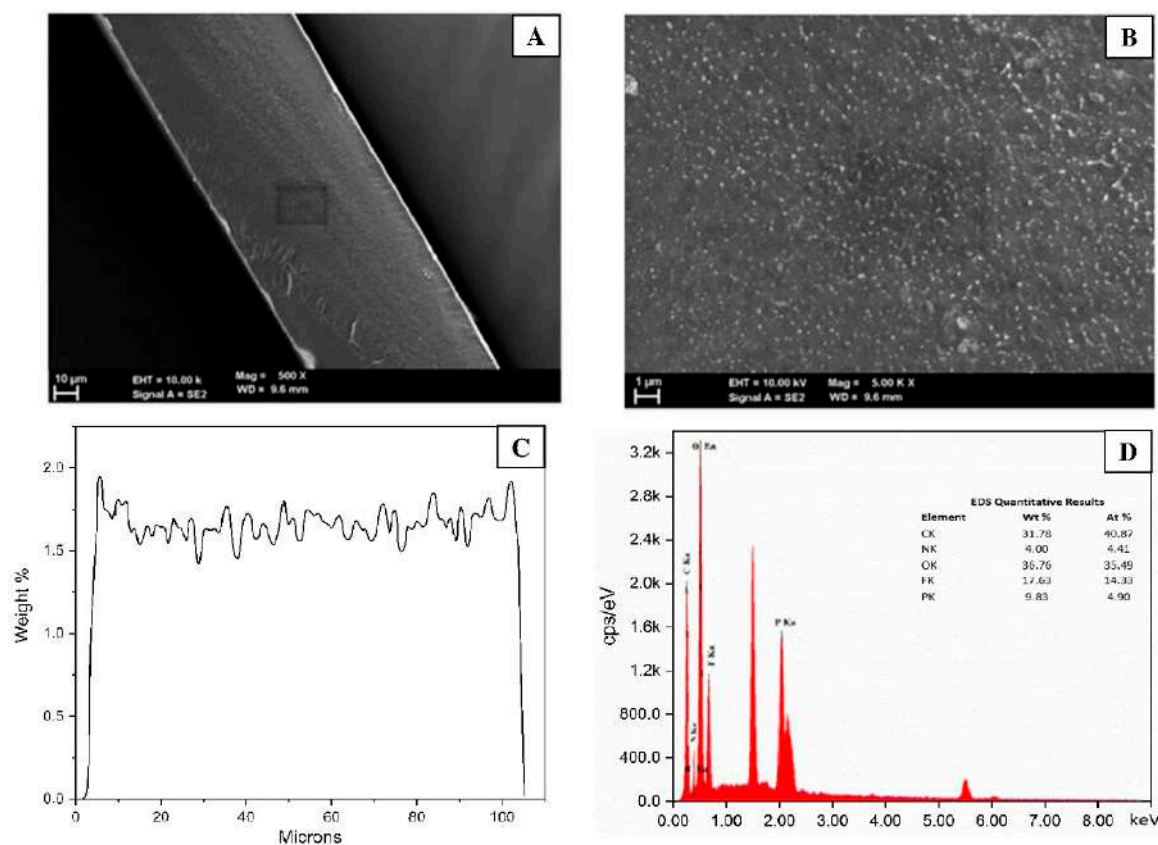
Figure 8. Cross-sectional view of ETFE-g-P(4-VP/1-VIm)/PA membrane with: (A) low magnification, (B) high magnification and (C) phosphorus mapping across membrane together with (D) EDX image of membrane elemental composition.
