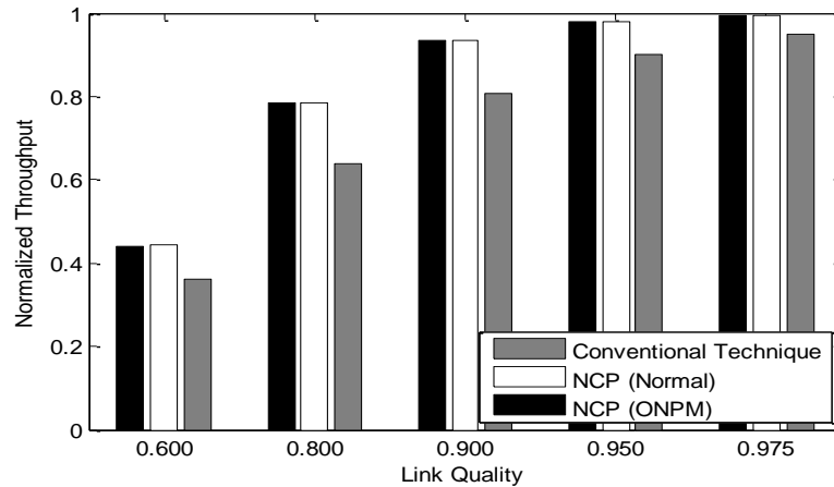
Figure 17. System throughput at different link qualities for \varepsilon \approx 1.3\varepsilon_{mi}
