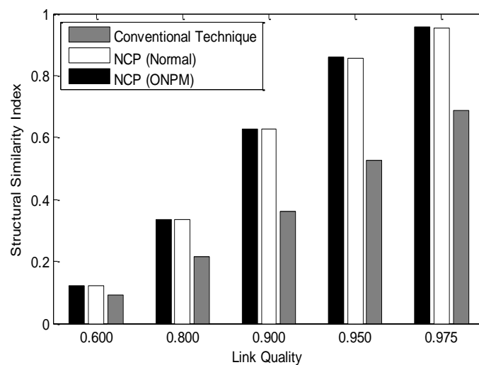
Figure 14. Quality of image at different link qualities for \varepsilon \approx 0.7\varepsilon_{\min}
