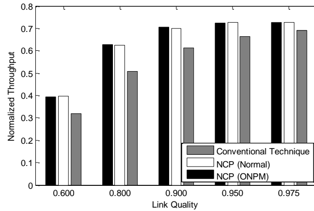
Figure 15. System throughput at different link qualities for \varepsilon \approx 0.7\varepsilon_{\min}
