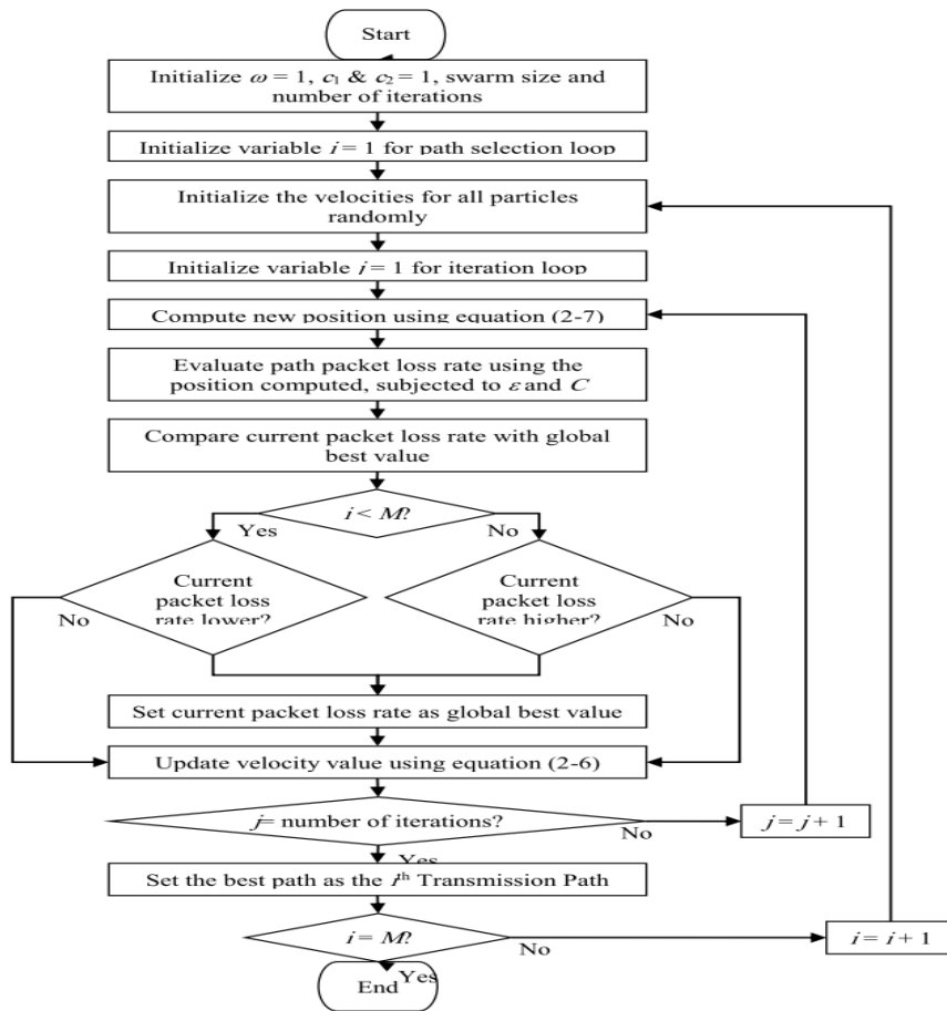
Figure 2. ONPM optimization process flow
