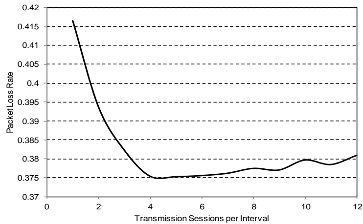
Figure 11 Packet loss rate for several Optimization Repetition Intervals
