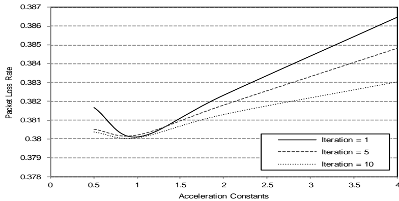
Figure 6. Packet loss rate for different acceleration constants in one particle swarm
