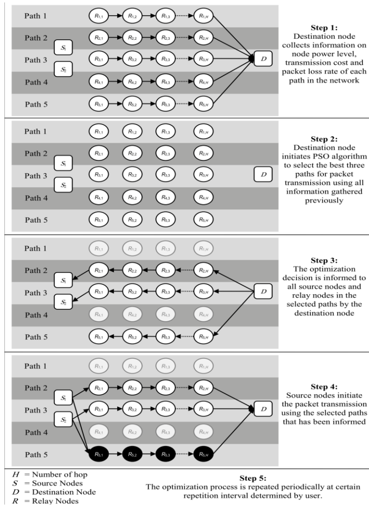
Figure 1. Process flows of ONPM in five paths network
