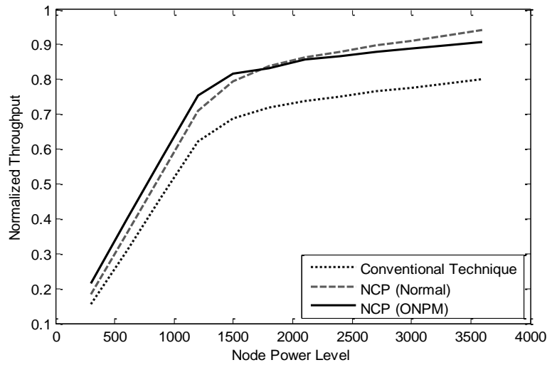
Figure 12. Throughput at different initial node power
