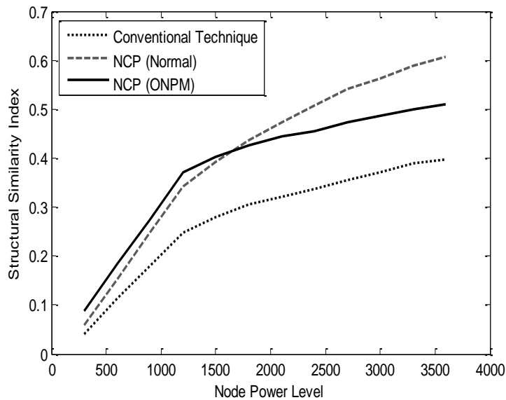
Figure 13. Effect of initial node power on image quality
