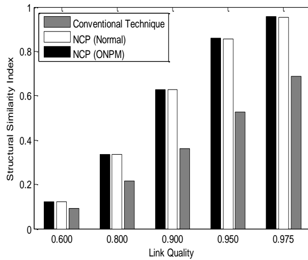
Figure 16. Quality of image at different link qualities for \varepsilon \approx 1.3\varepsilon_{\min}
