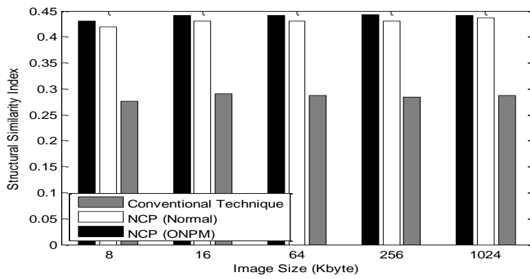
Figure 19. Effect of image size on the output image quality
