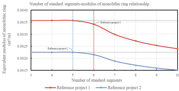
Figure 9 Relationship of number of standard segments with the equivalent flexural modulus of monolithic ring for the reference projects at 80% joint thickness
