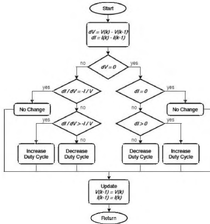
Fig. 1. IncCond method
