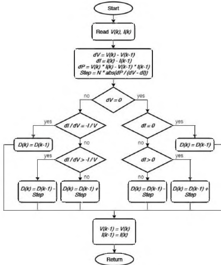
Fig. 2. IncCond step-size variable flowchart
