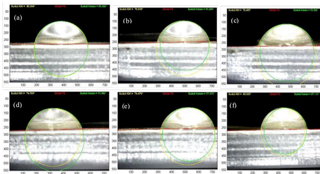
Fig. 3. The Contact angle of membranes: (a) Psf, (b-d) GO-Fe 3 O 4 /Psf untuk GO-Fe 3 O 4 (%Wt): 0.25%, 0.50%, 0.75%, and 1.0%; and (f) GO (0.5%)/Psf
