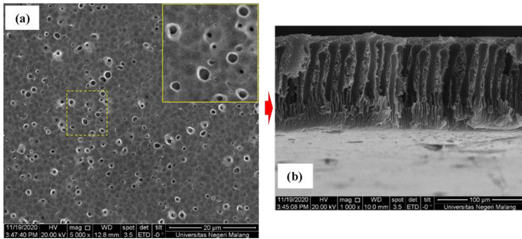
Fig. 6. Morphology of GO /PSf membrane: (a) surface and zoom (insert) and (b) cross-section.
