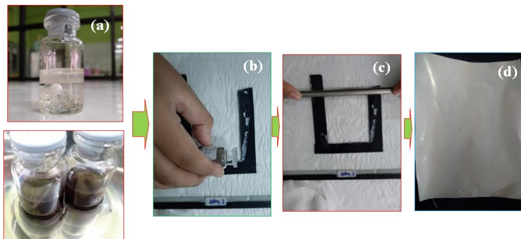
Fig. 1. Preparation of Psf, GO-Psf, and GO/Fe 3 O 4 -Psf membranes: (a) homogeneous solution, (b-c) membrane molding process, and (d) produced membrane.
