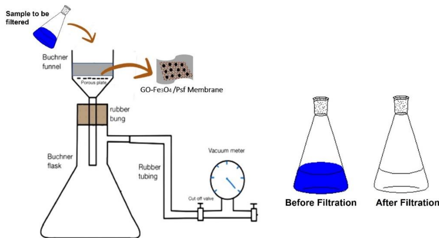
Fig. 7. The Filtration test with NaCl and MB
