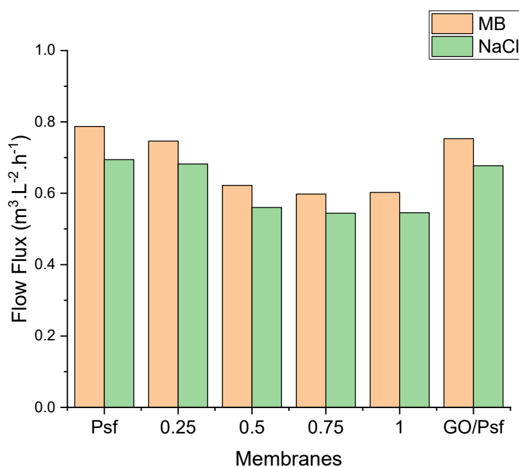
Fig. 8. Flow flux of methylene-blue and NaCl solution for GO- Fe 3 O 4 /PFs membranes.
