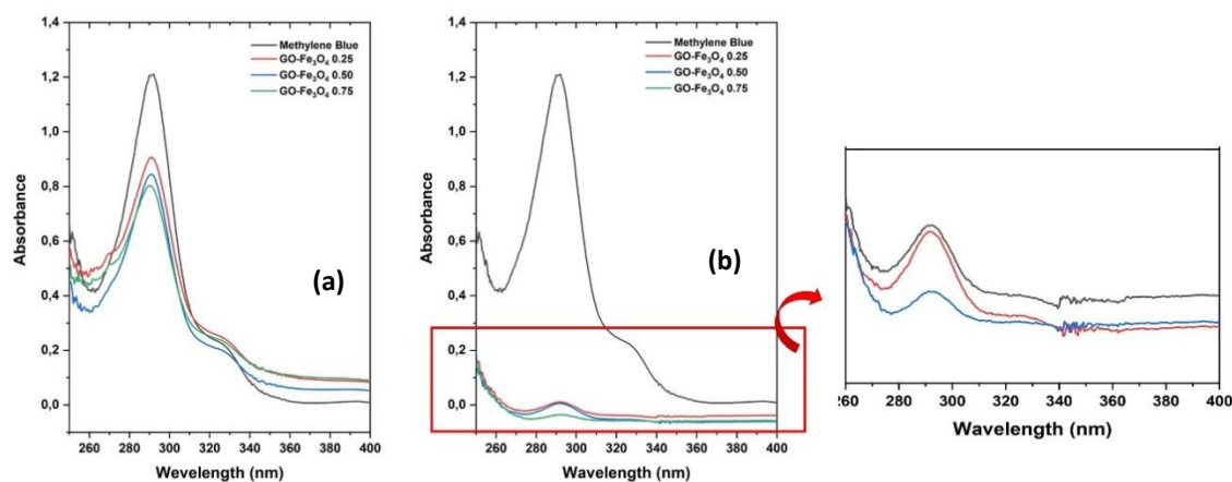
Fig. 9. UV-VIS of methylene blue filtration by GO-Fe 3 O 4 /Psf membranes: (a) one-time and (b) fifth time.
