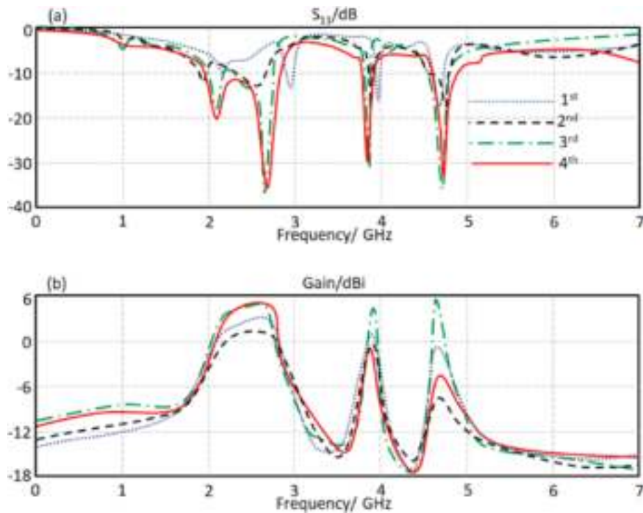
Fig. 5. Antenna array's performance as a function of staircase step number: (a) reflection coefficient ( S_{11} ), and (b) antenna gain.
