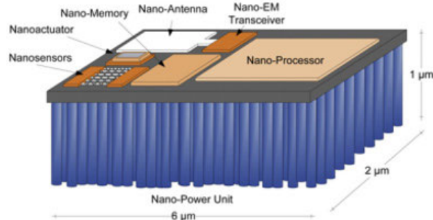
FIGURE 9. Nano-scale device [216].
