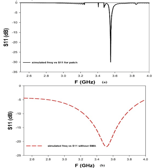
Figure 2. S11 of the planar antenna at (3.5GHz): (a)for patch (b)without (SMA).
