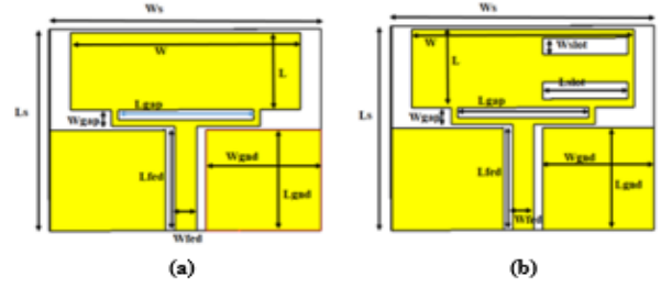
Figure 1. Planar microstrip antenna is presented. (a) general patch, (b) two-slot customized patch.
