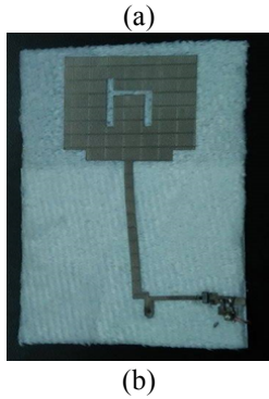
Figure 3. The (a) schematic and (b) the prototype of the rectenna.
