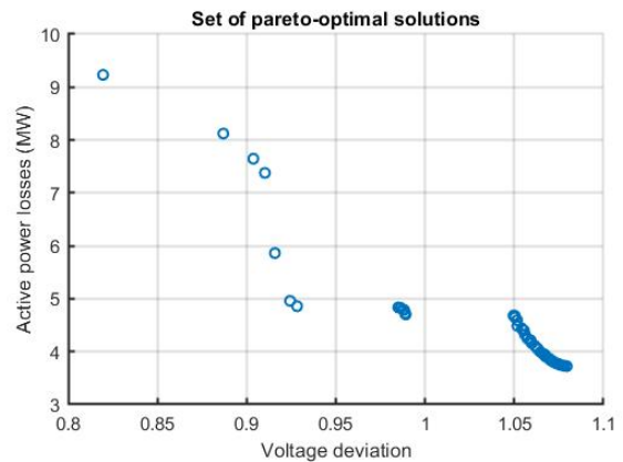
Figure 2. Pareto optimal solutions for 14-bus system
