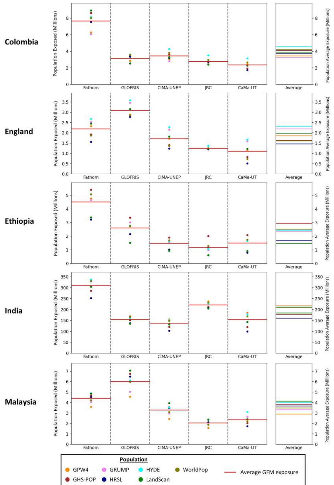
Figure 2. National flood exposure dot plots. Thirty five national flood exposure estimates calculated using five global flood models and seven global population data sets. Column on the right shows the average national flood exposure estimate calculated with each population data set.
