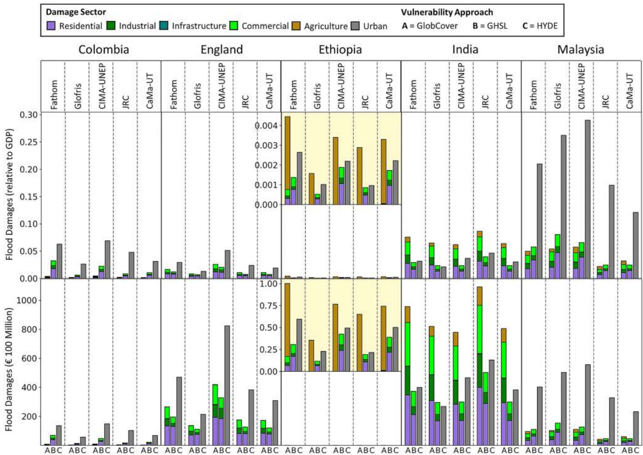
Figure 4. National flood damages calculated using five global flood models and three vulnerability approaches. (Top row) Normalized national flood damages (relative to national GDP). (Bottom row) Total national flood damages. Damages in 2010 Euros.
