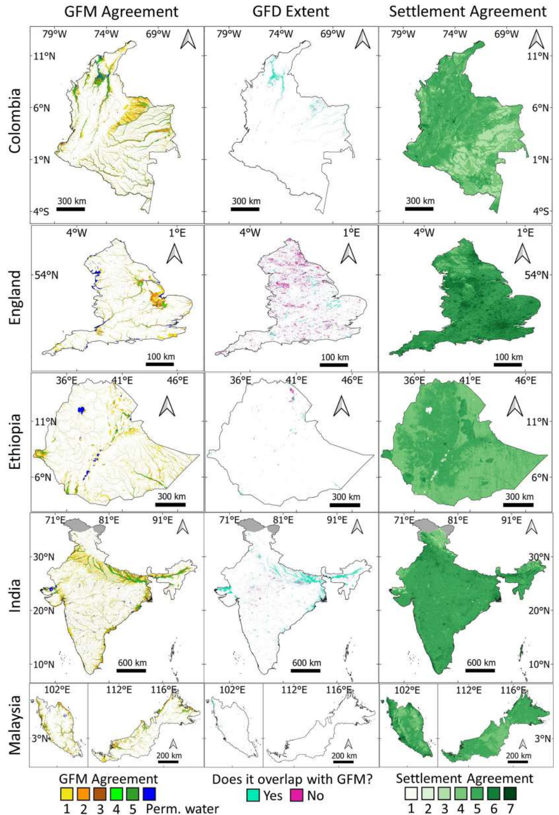
Figure 1. Maps of Global Flood Model (GFM) agreement, Global Flood Database (GFD) observed maximum flood extent and where it overlaps with any GFM, and global population data settlement agreement. Gray areas indicate no-data regions.
