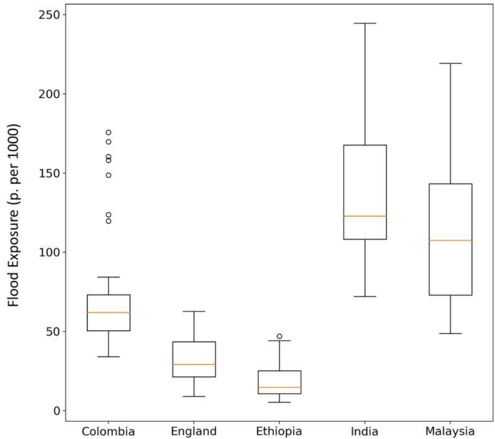
Figure 3. Box and whisker plots of normalized national flood exposure estimates for all five countries. Boxes represent the interquartile range (25th–75th quantiles), horizontal yellow lines represent the median normalized flood exposure, and points outside the whisker plot depict outliers (outside 1.5 times the interquartile range above or below the upper and lower quantiles).
