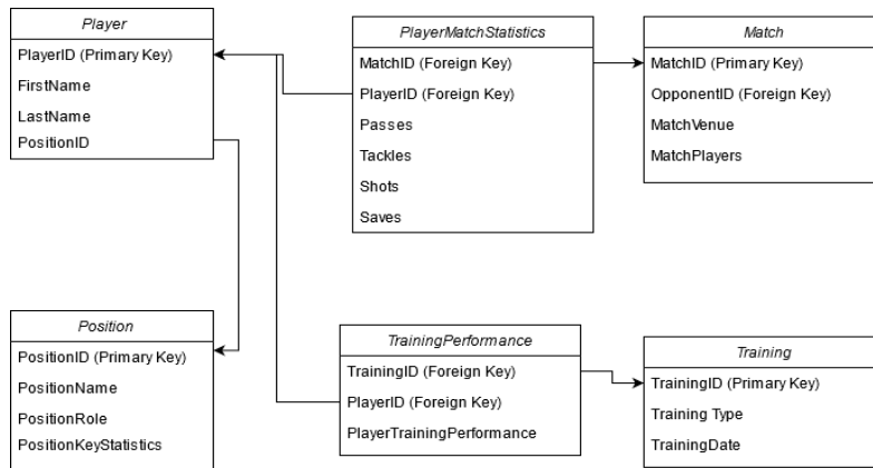
Fig. 4 - Example of a football data relational database scheme
