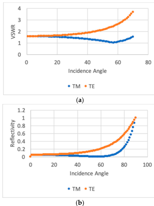
Figure 3. (a) VSWR for TE and TM polarizations in the UV region at the air–keratin interface. VSWR, which is measured from one to five, is higher than one for all incidence angles in the case of TE polarization. At the resonance frequency, the VSWR is close to one, corresponding to Brewster’s angle condition or equivalently zero reflectivity for TM polarization. (b). Reflectivity spectrum for TE and TM polarizations in the UV region at the air–keratin interface. We can observe that both graphs displayed correlate with each other.
