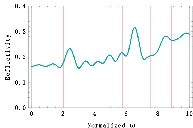
Figure 6. Theoretical reflectivity spectrum of the simulated feather for TE polarization and incidence angle of 57^\circ . Four high reflectivity bands shifted towards the UV region. The red lines at 1237 nm, 437 nm, 333 nm, and 284 nm represented the positions of the peaks when the angle of incidence was 0^\circ . The average reflectivity from 300 to 700 nm increased up to 21.1 \pm 4.5\% . A UV-chroma of 30% was calculated in the same range. The normalized frequency is given by \omega = 2\pi(dl + dm)/\lambda .
