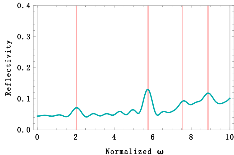
Figure 5. Theoretical reflectivity spectrum of the simulated barbule feather for TE, TM polarization, and incidence angle of 0^\circ . Four high reflectivity bands (red lines) can be observed at 1237 nm, 437 nm, 333 nm, and 284 nm. The average reflectivity from 300 to 700 nm was 6.7 \pm 2.3\% , close to the experimental value of 6.4 \pm 0.39\% measured in [10]. A UV-chroma of 27% was calculated in the same range, and a UV-chroma of 24 \pm 0.19\% was reported in [10]. The normalized frequency is given by \omega = 2\pi(dl + dm)/\lambda .
