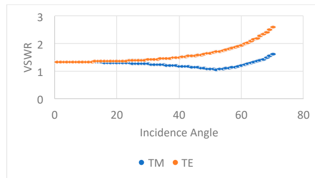
Figure 4. VSWR for TE and TM polarizations in the UV region at the keratin–melanin interface; VSWR is higher than one for all incidence angles. From our simulation results, VSWR values go from one to five. At resonance, the VSWR is close to one, corresponding to Brewster’s angle condition or equivalently zero reflectivity for TM polarization.
