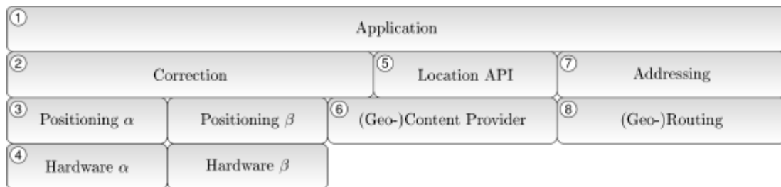
Figure 3 Layered Architecture of ILBS [12]
