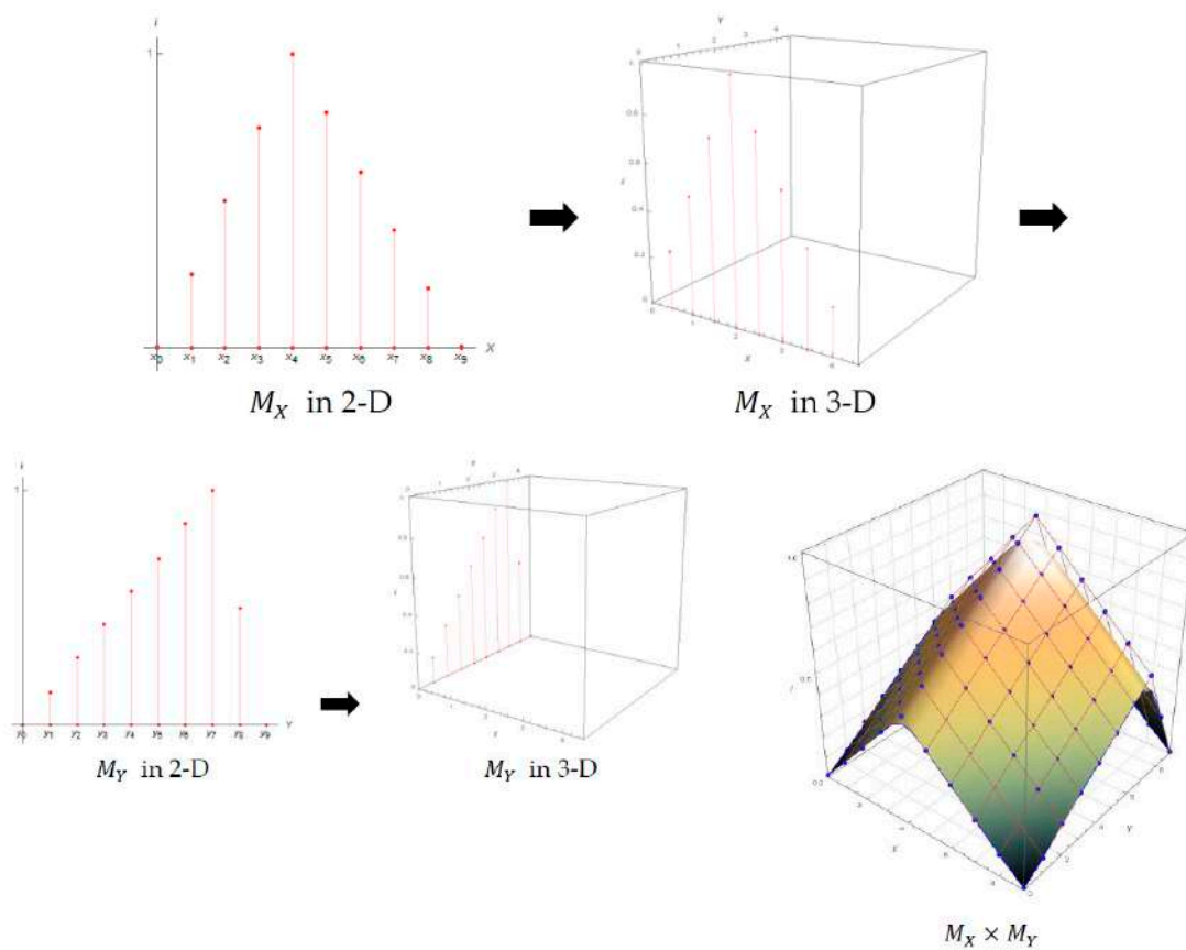
Figure 10. Fuzzy linguistic point relation of medium linguistic functions M_X and M_Y .
