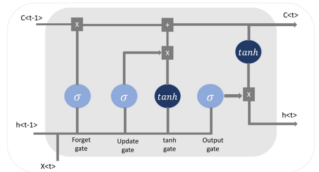
FIGURE 4. LSTM structure.
