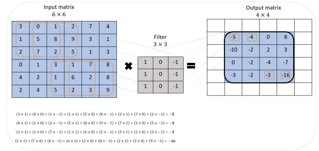
FIGURE 3. Convolution process.
