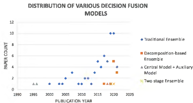
FIGURE 10. Distribution of decision fusion models.
