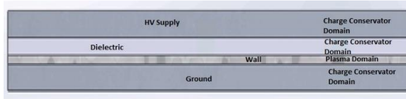
Fig. 4. Simulation boundary conditions for ozone plasma generation.
