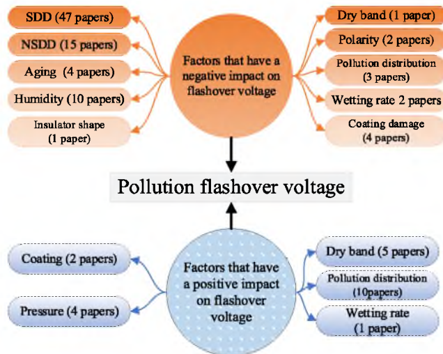
FIGURE 27. Flashover voltage factors and their impact classification.
