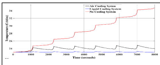
Figure 6: Battery temperature of different cooling system (NEDC)
