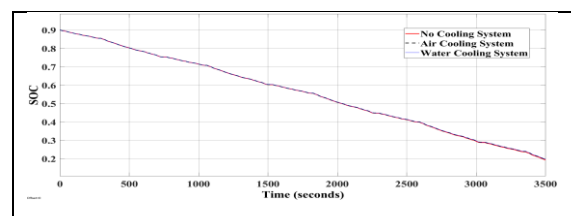
Figure 9: SOC of battery under HWFET analysis
