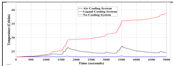
Figure 8: Battery temperature of different cooling system (WLTC)
