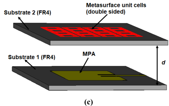
FIGURE 7. The proposed metasurface antenna configuration. (a), (b) Front and Back view of Antenna dimensions, respectively. (c) Metasurface placed above the antenna.
