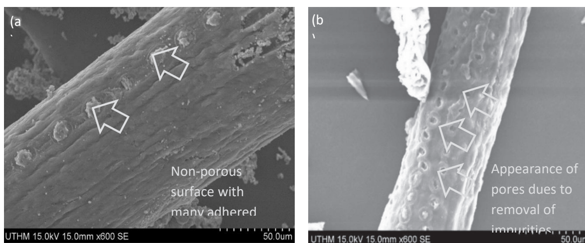
FIGURE 2. SEM images of (a) Raw PEFB and (b) Pre-treated PEFB
