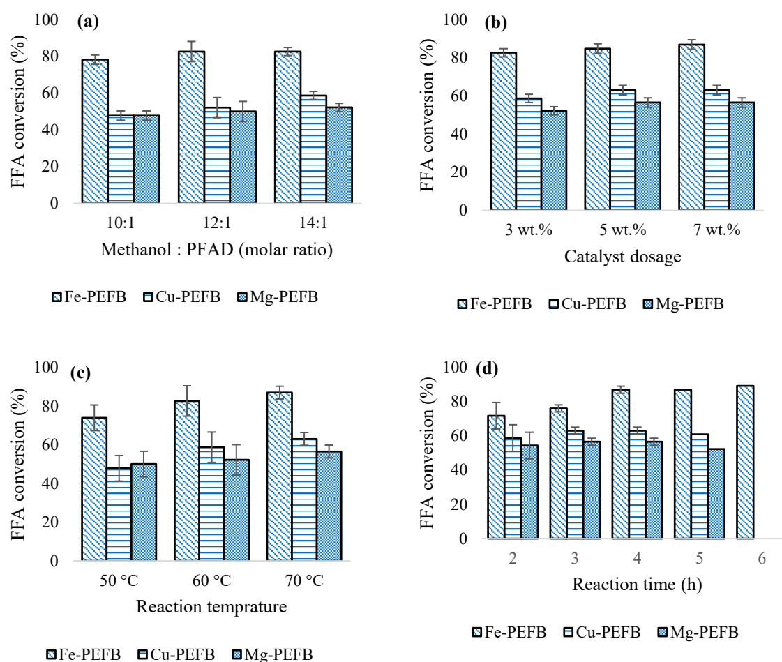
FIGURE 6. Optimization of the process parameters; (a) Effect of methanol : PFAD mole ratio (10:1, 12:1, 14:1) on FFA conversion (%) (catalyst dosage 3 wt%, 4 h reaction time at 70 °C), (b) Effect of catalyst dosage (3, 5, 7 wt%) on FFA conversion (%) (methanol: PFAD mole ratio 14:1, 4 h reaction time at 70 °C), (c) Effect of reaction temperature (50, 60, and 70 °C) on FFA conversion (%) (methanol: PFAD mole ratio 14:1, catalyst dosage 7 wt% Fe-PEFB and 5 wt% Cu and Mg-PEFB, 4 h reaction time), and (d) Effect of reaction time (2 - 6 h) on FFA conversion (%) (methanol: PFAD mole ratio 14:1, catalyst dosage 7 wt% of Fe-PEFB and 5 wt% of Cu and Mg-PEFB at 70 °C)
