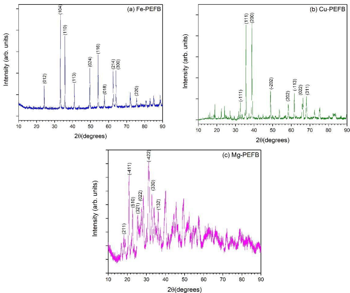
FIGURE 1. XRD patterns of (a) Fe-PEFB, (b) Cu-PEFB, and (c) Mg-PEFB
