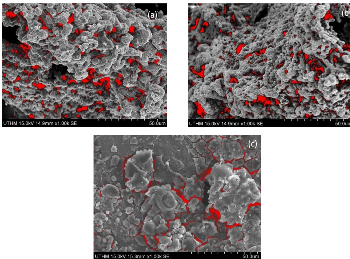
FIGURE 3. SEM images of (a) Fe-PEFB, (b) Cu-PEFB and (c) Mg-PEFB where the red color indicates pores
