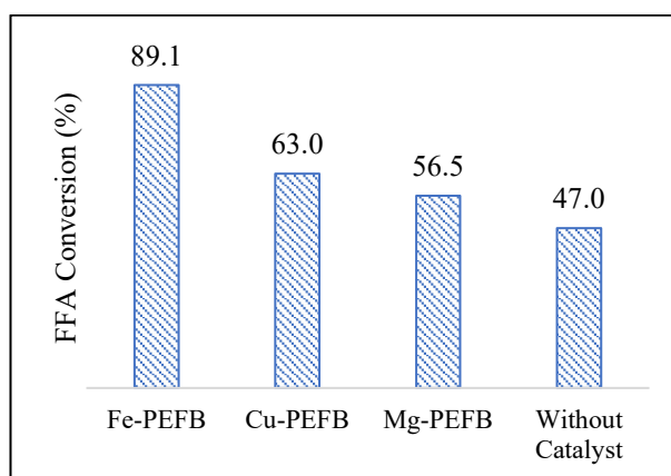
FIGURE 5. Comparison of FFA Conversion (%) achieved with and without catalysts
