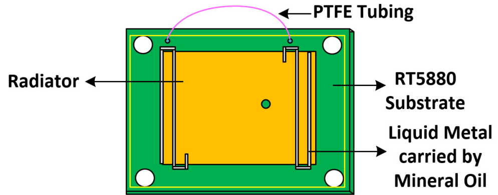
Figure 17. The picture of the microfluidic structure.
