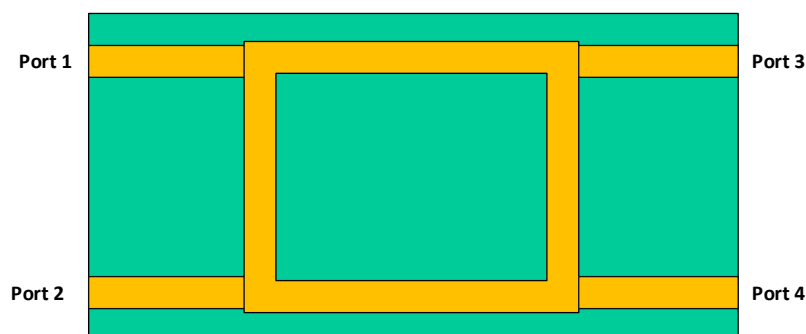
Figure 1. Diagram of the tunable branch line coupler (BLC).
