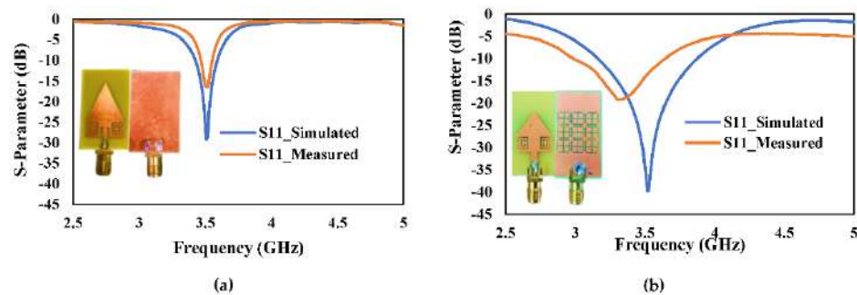
Figure 16. Simulated and Measured S-Parameter response (a) Proposed antenna with the complete ground plane (b) Proposed antenna with 3 \times 3 cross-slot MTM structure etched on the ground plane.
