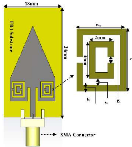
Figure 3. Layout of proposed antenna design.
