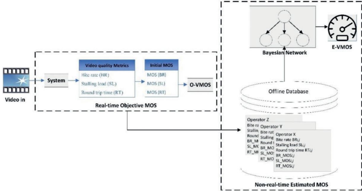
Figure 5: A general framework of estimated MOS process
