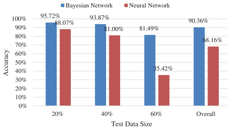
Figure 13: Accuracy comparison between bayesian and neural networks
