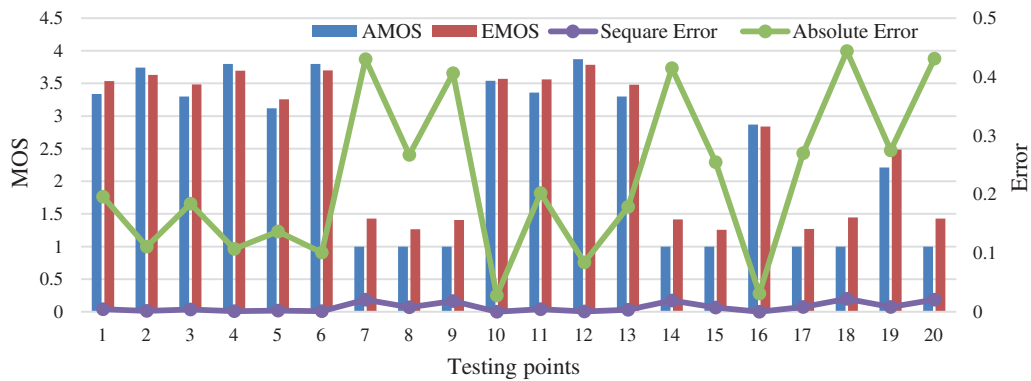
Figure 11: Graph bar of AMOS, EMOS with absolute and squared error against random test points
