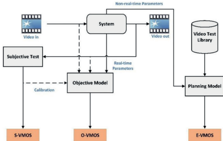
Figure 1: Relationship between VMOS identifiers [2]
