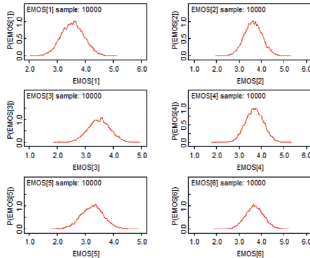
Figure 9: Kernel density of six EMOS nodes
