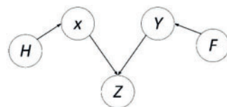
Figure 3: Directed acyclic graph
