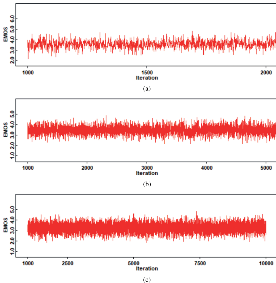
Figure 7: Generated samples of EMOS value (a) 2000 iterations (b) 5000 iterations (c) 10000 iterations
