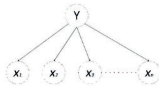
Figure 2: Basic concept of the Bayesian graphical model
