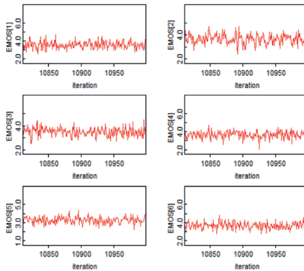
Figure 8: Dynamic tracing of six EMOS nodes
