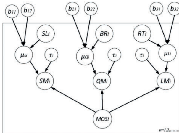
Figure 4: Proposed Bayesian network model for estimating MOS
