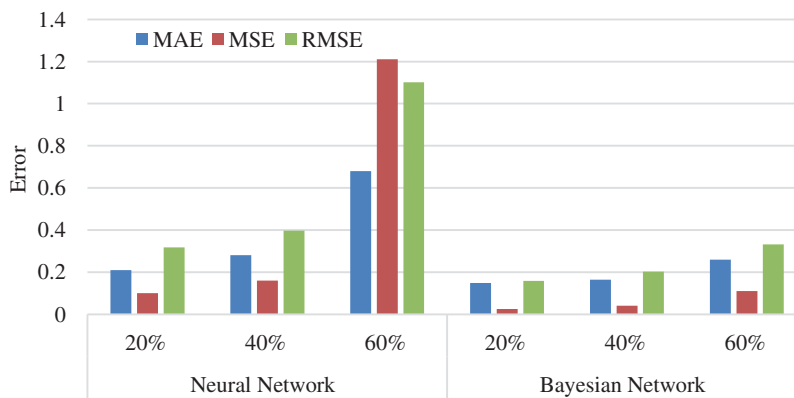
Figure 12: Comparison between bayesian and neural networks over test data sizes
