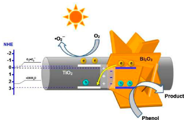
Figure 11. Schematic mechanism of phenol removal by photocatalysis using \text{Bi}_2\text{O}_3/\text{TiO}_2 NFs [92]. Reproduced with permission from Elsevier, 2022.
