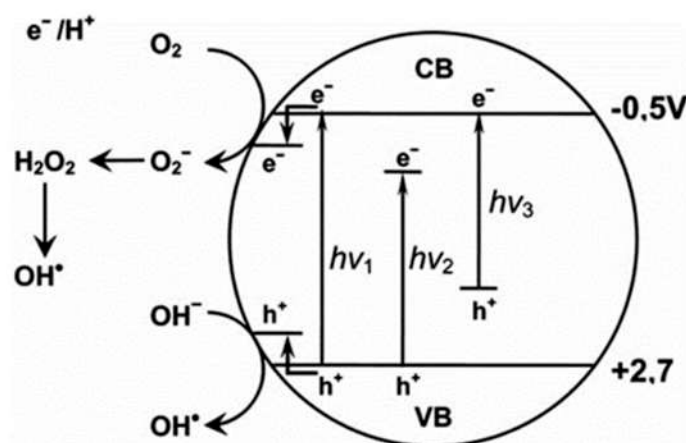
Figure 6. Representative scheme of photocatalysis process of TiO 2 . hv 1 : pristine TiO 2 ; hv 2 : metal-doped TiO 2 ; and hv 3 : nonmetaldoped TiO 2 [65]. Reproduced with permission from Eureka Science (FZC), 2022.
