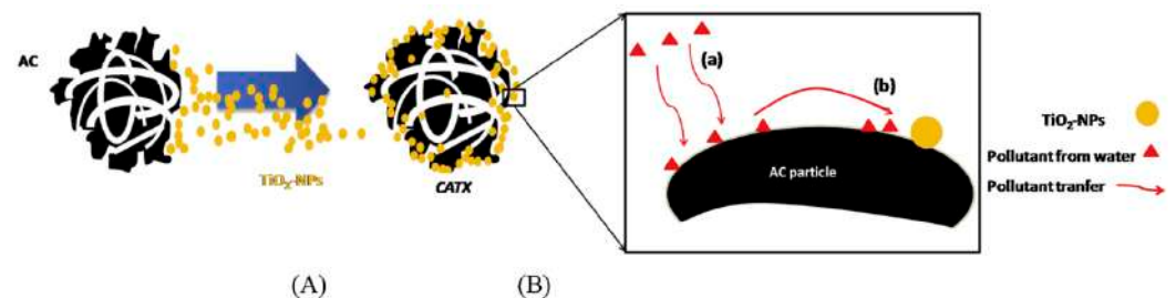
Figure 9. Scheme of (A) TiO 2 impregnation at the external porosity of AC support by surface coating (CATX, X referred to %wt of TiO 2 ) and (B) pollutant transfer towards photocatalytic center [87]. Reproduced with permission from Elsevier, 2022.
