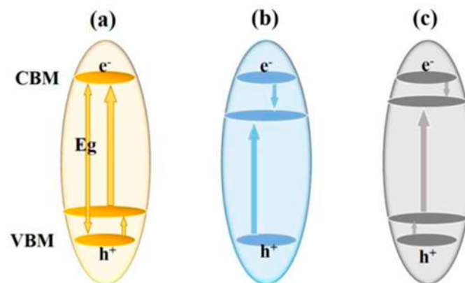
Figure 5. Representative mechanisms of the energy band engineering of \text{TiO}_2 : (a) a higher shift in valence band maximum (VBM); (b) a lower shift in conduction band minimum (CBM); and (c) continuous modification of both VBM and CBM [56].
