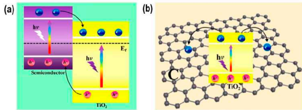
Figure 8. (a) Charge carrier migration mechanism of TiO 2 -based nanocomposite material, including trapping on TiO 2 and the second phase/component and (b) TiO 2 intercalation on the support material (example: graphene), which increases the light absorption region and intensity, charge carrier life-time, and absorptivity toward organic pollutants [81].
