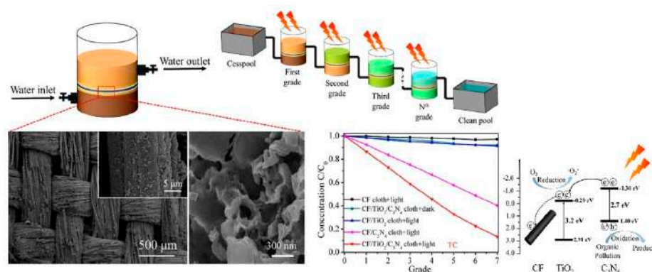
Figure 15. Summary of the PM process using a TiO 2 /C 3 N 4 /CF cloth filter membrane for pollutant degradation under light radiation with high desired morphological, good performance, and schematic mechanism of electron-hole separation [104]. Reproduced with permission from Elsevier, 2022.
