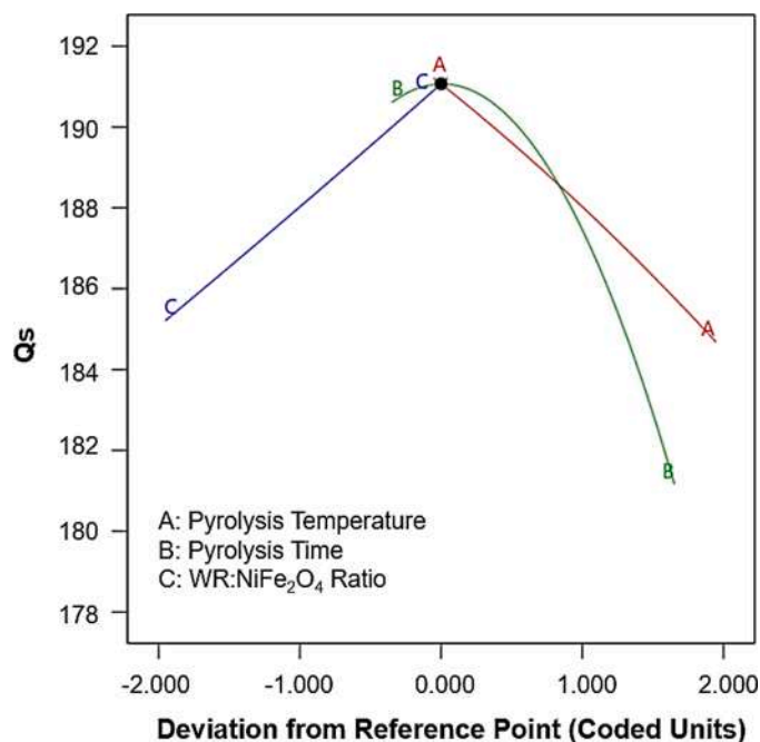
Fig. 5. Effect of perturbation for each process variables in BCWR synthesis.
